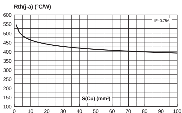
Fig. 9: Thermal resistance junction to ambient versus copper surface (epoxy printed circuit board FR4, copper thickness: 35μm).
