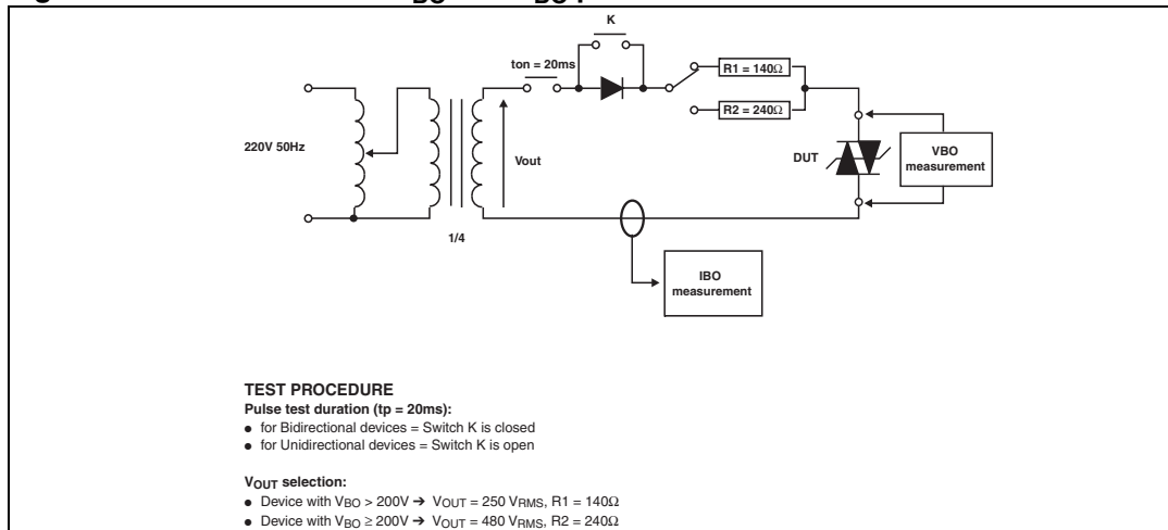
Figure 10. Test circuit 2 for I_{BO} and V_{BO} parameters
