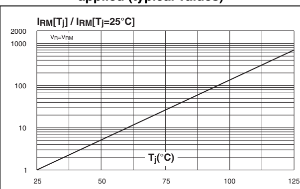
Figure 6. Relative variation of leakage current versus reverse voltage applied (typical values)
