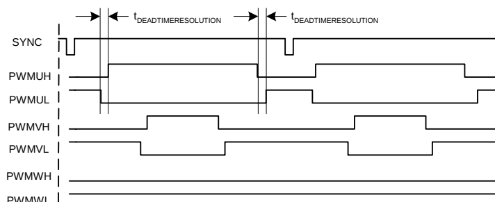
Figure 12: PWM Timing
