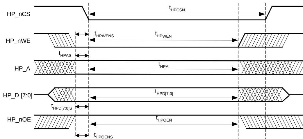
Figure 10: Host Parallel Write Cycle
