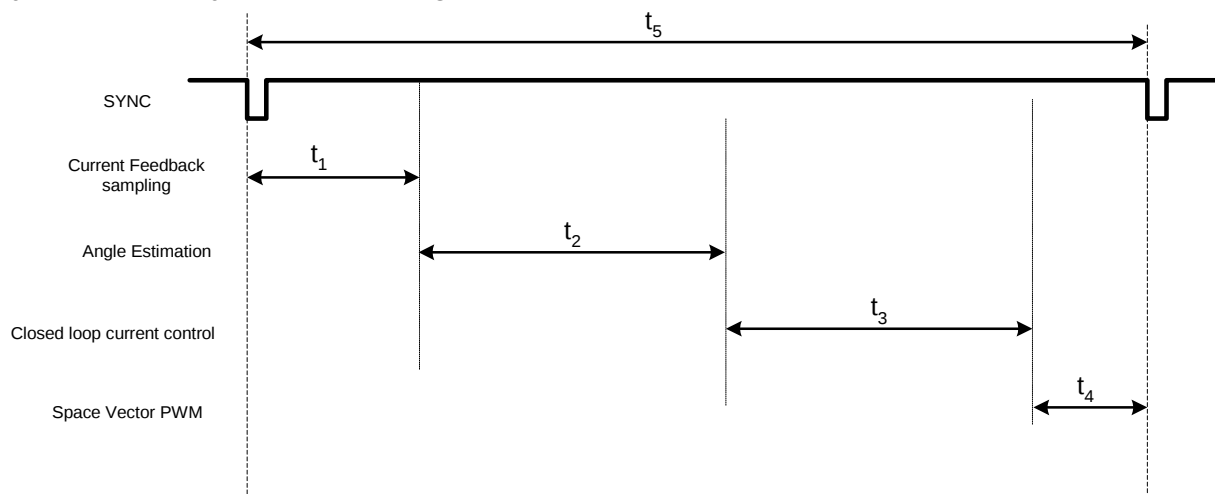
Figure 6: System Level SYNC To SYNC Timing
