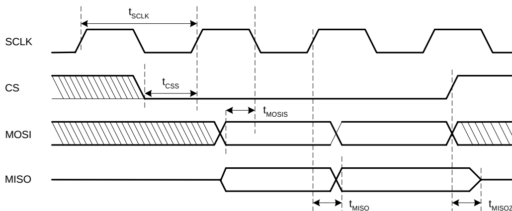
Figure 8: SPI Timing
