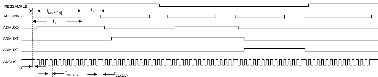
Figure 14: Top Level ADC Timing
