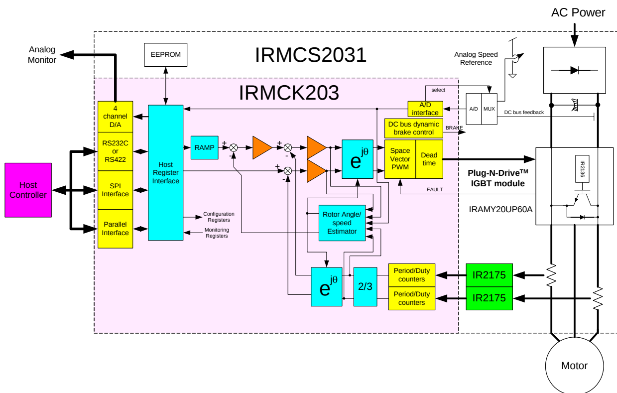
Figure 1: IRMCK203 Simplified Blocks
