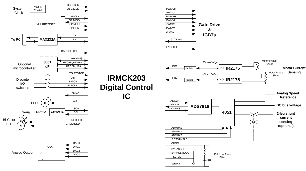
Figure 3: Application Connection of IRMCK203
