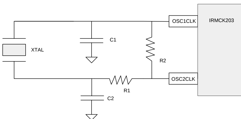
Figure 4: Oscillator Circuit
