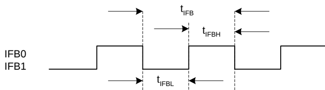
Figure 13: IR2175 Interface
