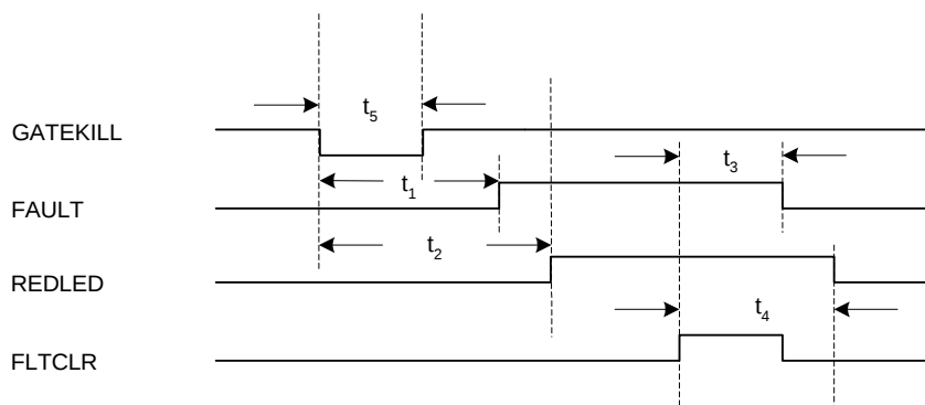
Figure 7: FAULT and REDLED Response to GATEKILL
