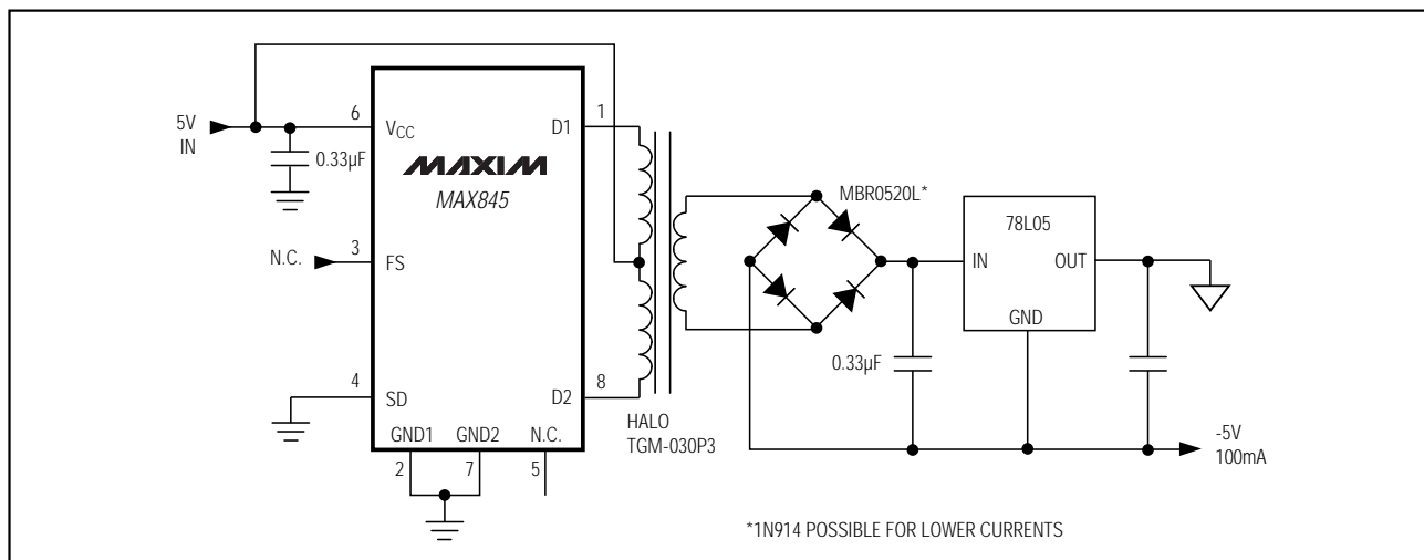
Figure 5. Low-Noise Supply
