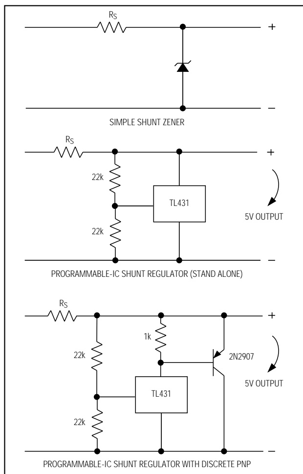
Figure 12. Shunt-Regulator Circuits
