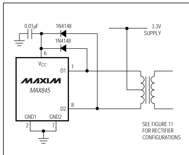
Figure 4. 3.3V Input to Isolated Output Application Circuit
