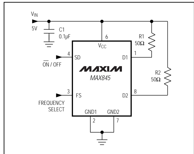
Figure 1. Test Circuit
