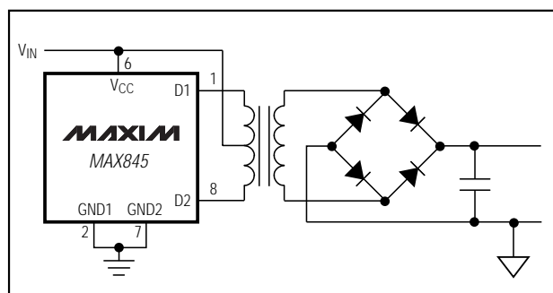
Figure 11b. 4-Diode Bridge
