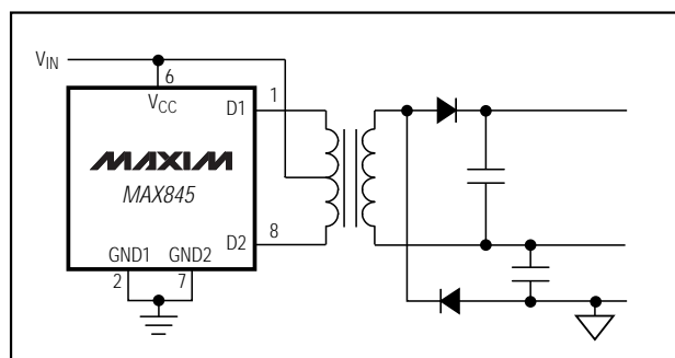
Figure 11c. Voltage Doubler
