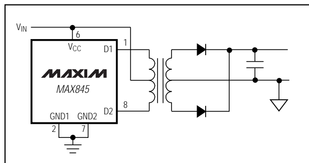
Figure 11a. 2-Diode Push-Pull
