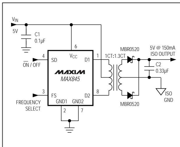
Figure 3. 5V to Isolated 5V Application Circuit
