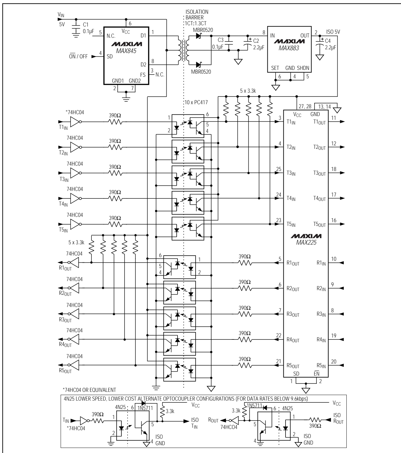
Figure 10. Typical RS-232 Application Circuit
