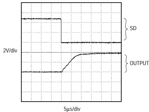
TIME FROM SHUTDOWN TO POWER-UP
