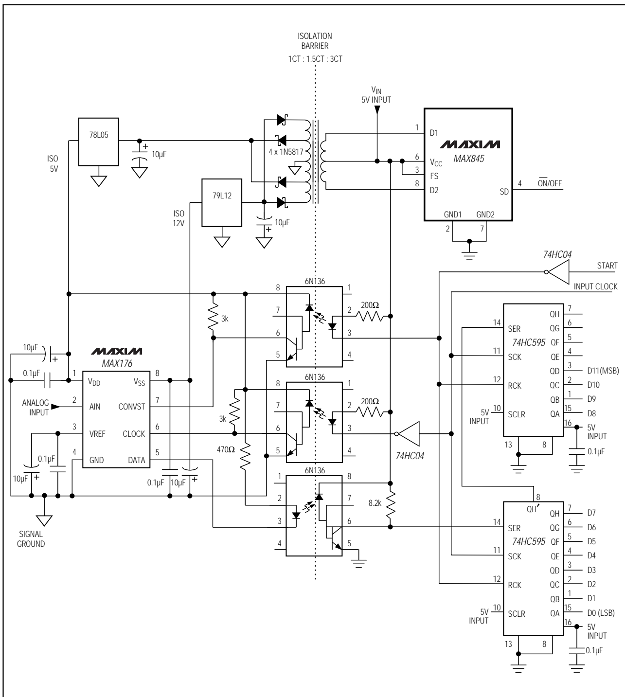
Figure 6. Typical Isolated Data-Conversion Application
