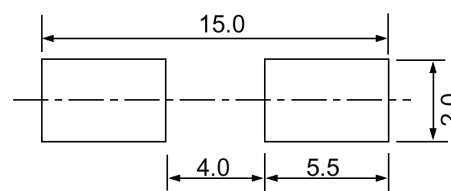
Figure 2) Suggested Land Pattern
