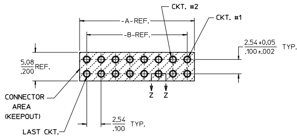
RECOMMENDED PCB LAYOUT (COMPONENT SIDE)
