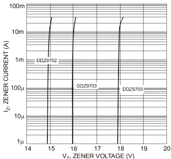
Fig. 6 Typical Zener Breakdown Characteristics, DDZ9702 - DDZ9705
