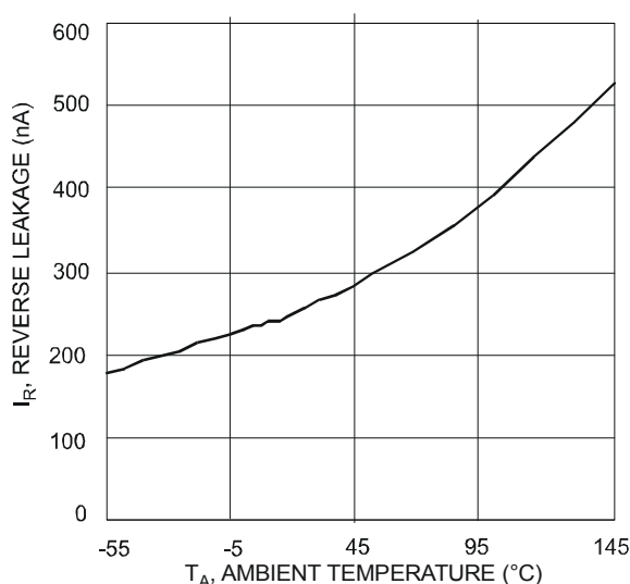
Fig. 21 Typical Leakage vs. Ambient Temperature, DDZ9681
