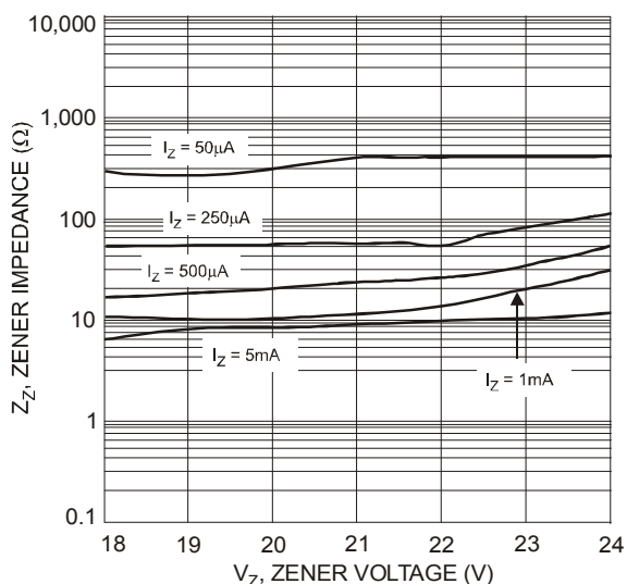
Fig. 14 Typical Zener Impedance Characteristics, DDZ9705 - DDZ9709
