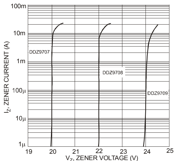
Fig. 7 Typical Zener Breakdown Characteristics, DDZ9707 - DDZ9709
