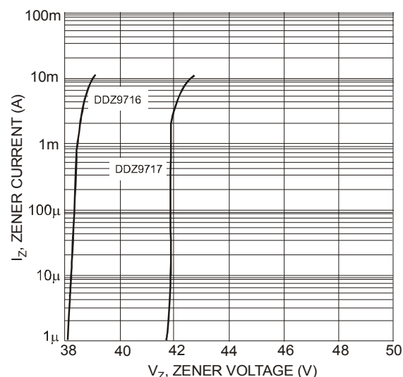
Fig. 9 Typical Zener Breakdown Characteristics, DDZ9716 - DDZ9717
