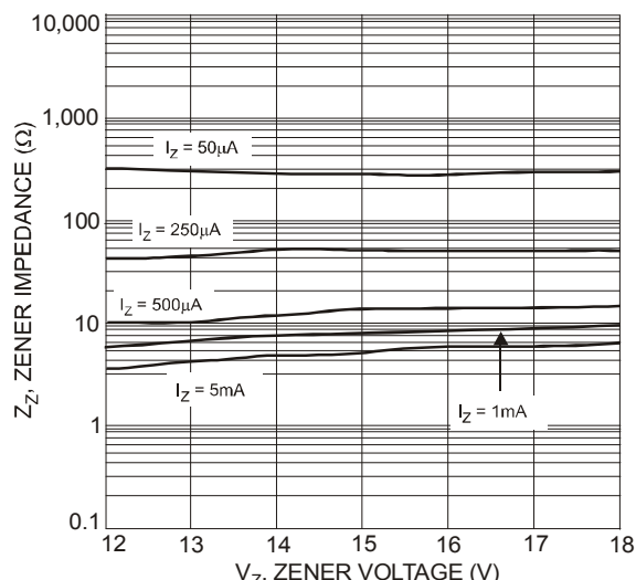
Fig. 13 Typical Zener Impedance Characteristics, DDZ9699 - DDZ9705
