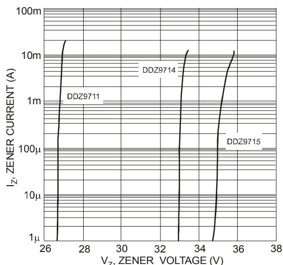
Fig. 8 Typical Zener Breakdown Characteristics, DDZ9711 - DDZ9715
