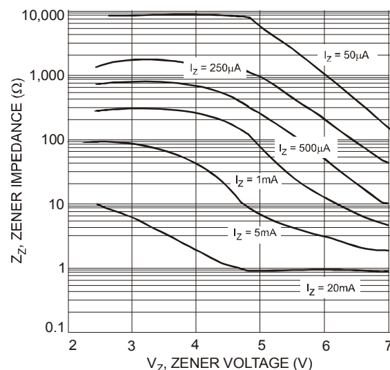
Fig. 11 Typical Zener Impedance Characteristics, DDZ9681 - DDZ9692
