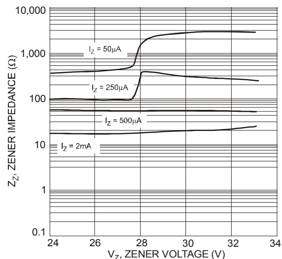
Fig. 15 Typical Zener Impedance Characteristics, DDZ9709 - DDZ9714
