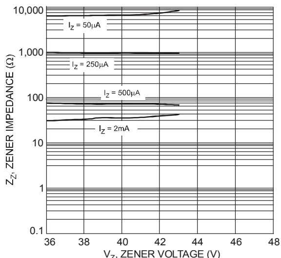
Fig. 16 Typical Zener Impedance Characteristics, DDZ9715 - DDZ9717
