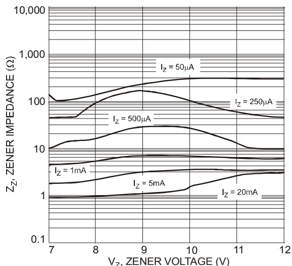
Fig. 12 Typical Zener Impedance Characteristics, DDZ9693 - DDZ9699
