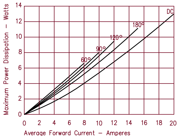
Figure 5 Maximum Forward Power Dissipation — Per Leg
