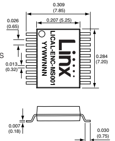
Figure 1: Package Dimensions
