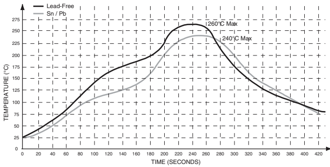
Figure 13: MS Series Reflow Profile
