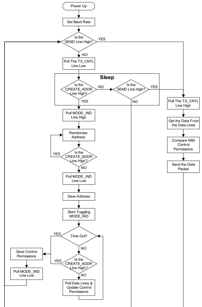
Figure 10: MS Series Encoder Flowchart
