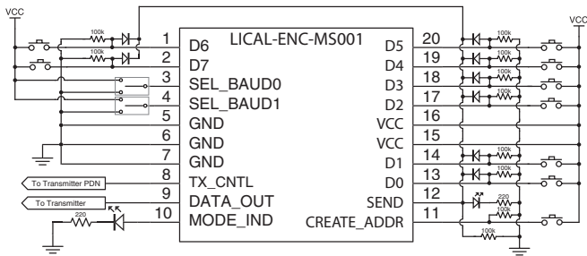
Figure 11: MS Series Encoder Application Circuit
