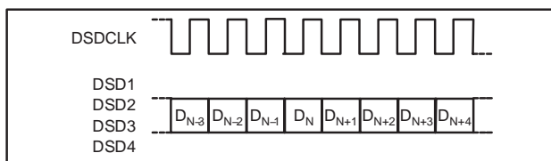
Figure 5. DSD Input and Output Data Format
