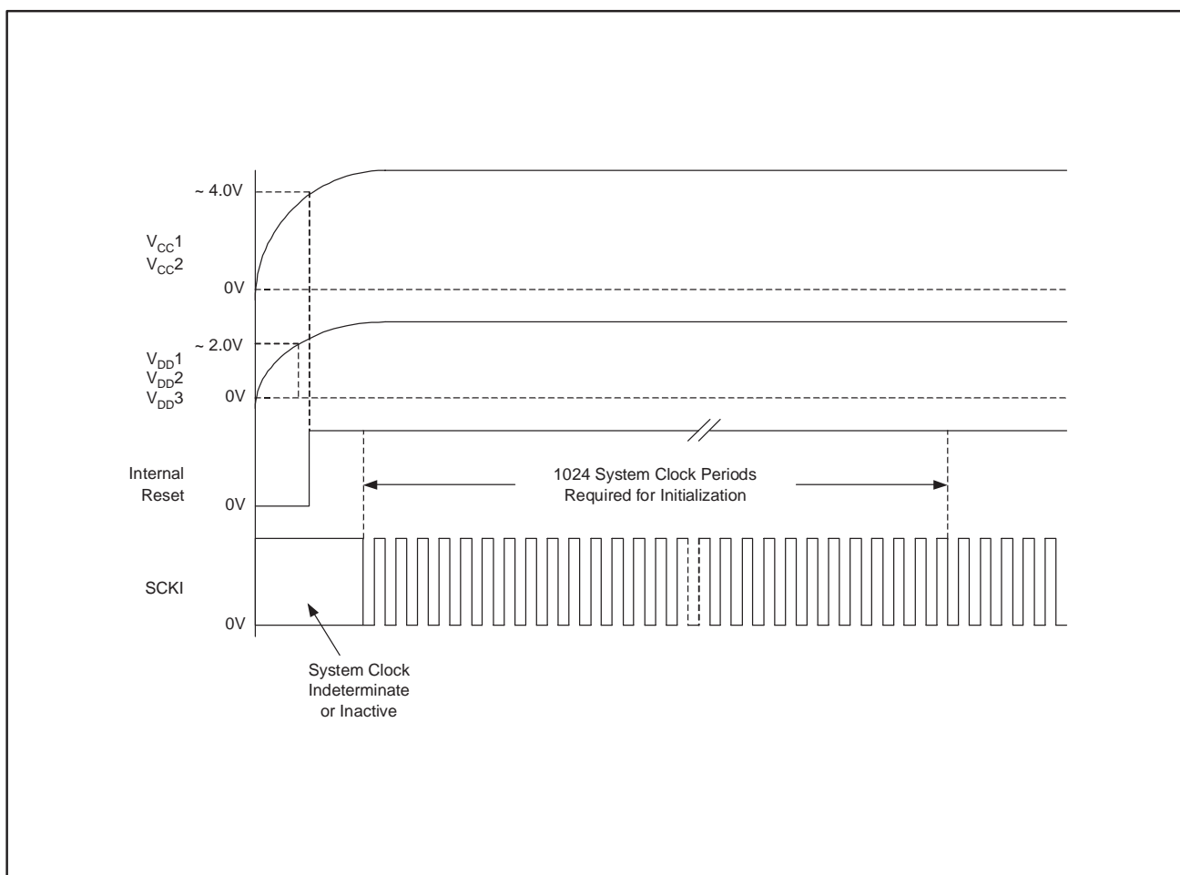
Figure 11. Power-On Reset Sequence
