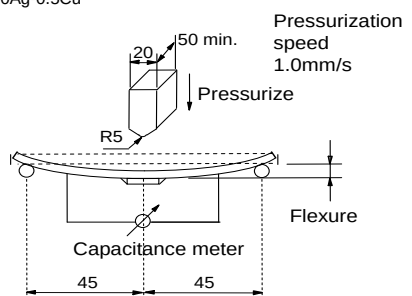
Fig.2 (in mm)
