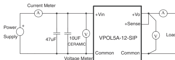
Figure 11. VPOL5A-12-SIP Test Setup
