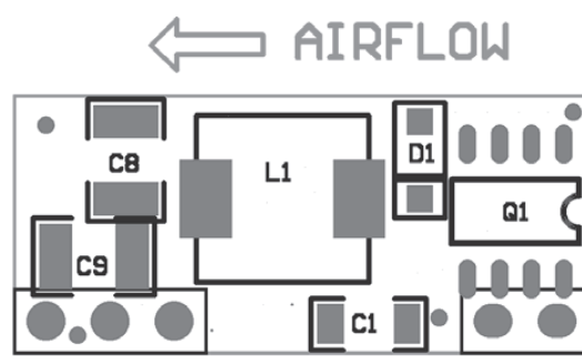
Figure 7. Temperature Measurement Location for VPOL5A-12-SIP
