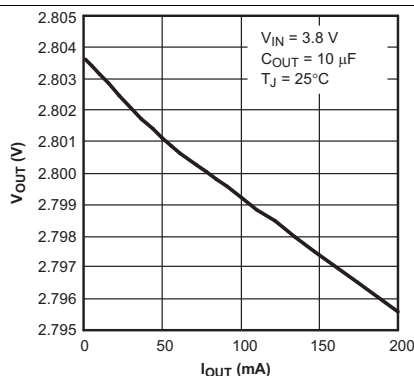
Figure 1. TPS73028 Output Voltage vs Output Current
