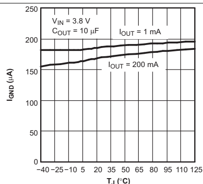
Figure 3. TPS73028 Ground Current vs Junction Temperature
