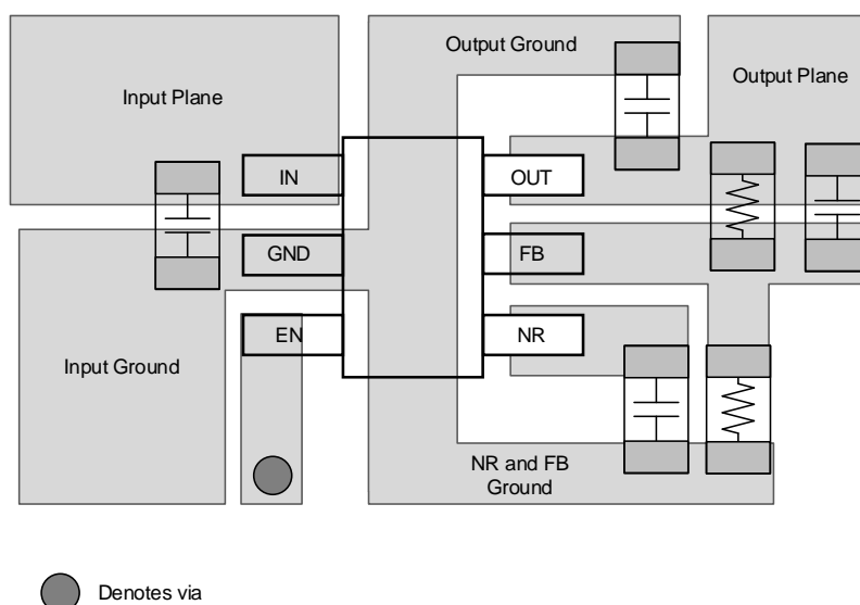
Figure 23. Layout Example (DBV Package)
