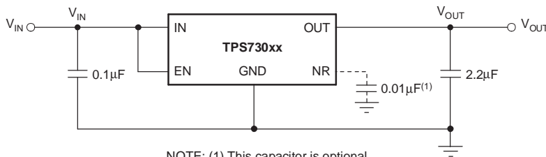
Figure 18. Typical Application Circuit
