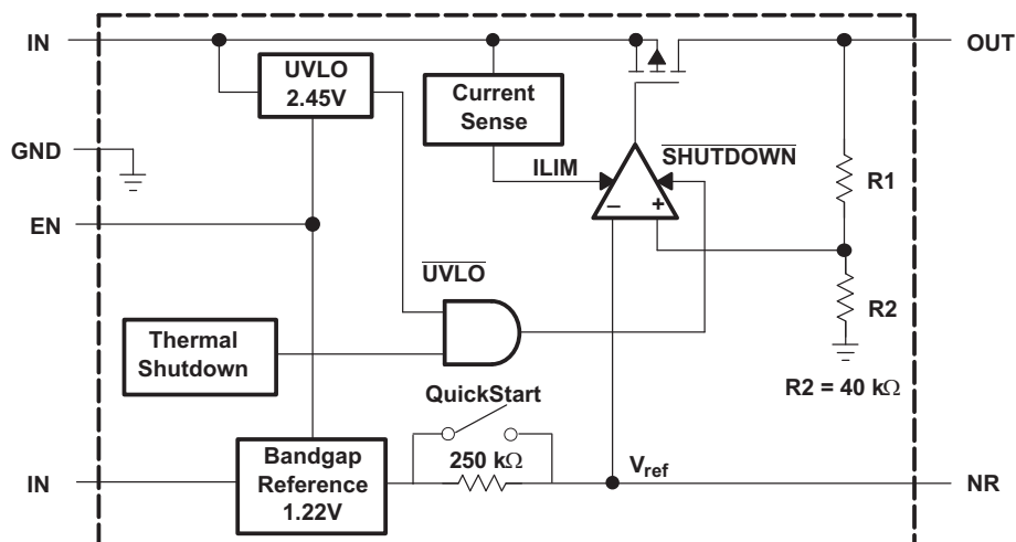
Figure 16. TPS730 Block Diagram (Fixed-Voltage Versions)
