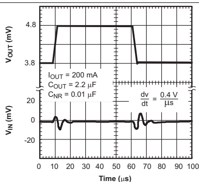
Figure 9. TPS73028 Line Transient Response
