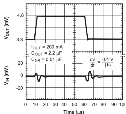
Figure 20. TPS73028 Line Transient Response
