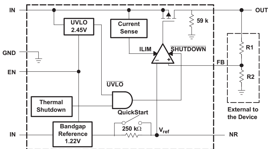
Figure 15. TPS730 Block Diagram (Adjustable-Voltage Version)
