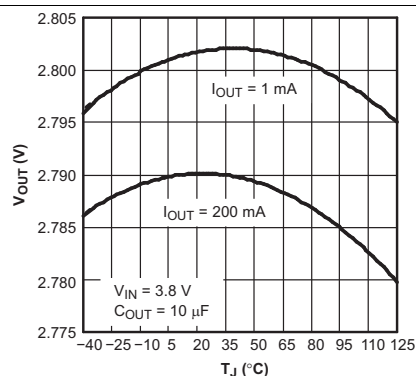
Figure 2. TPS73028 Output Voltage vs Junction Temperature
