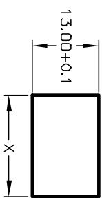
PANEL CUTOUT
