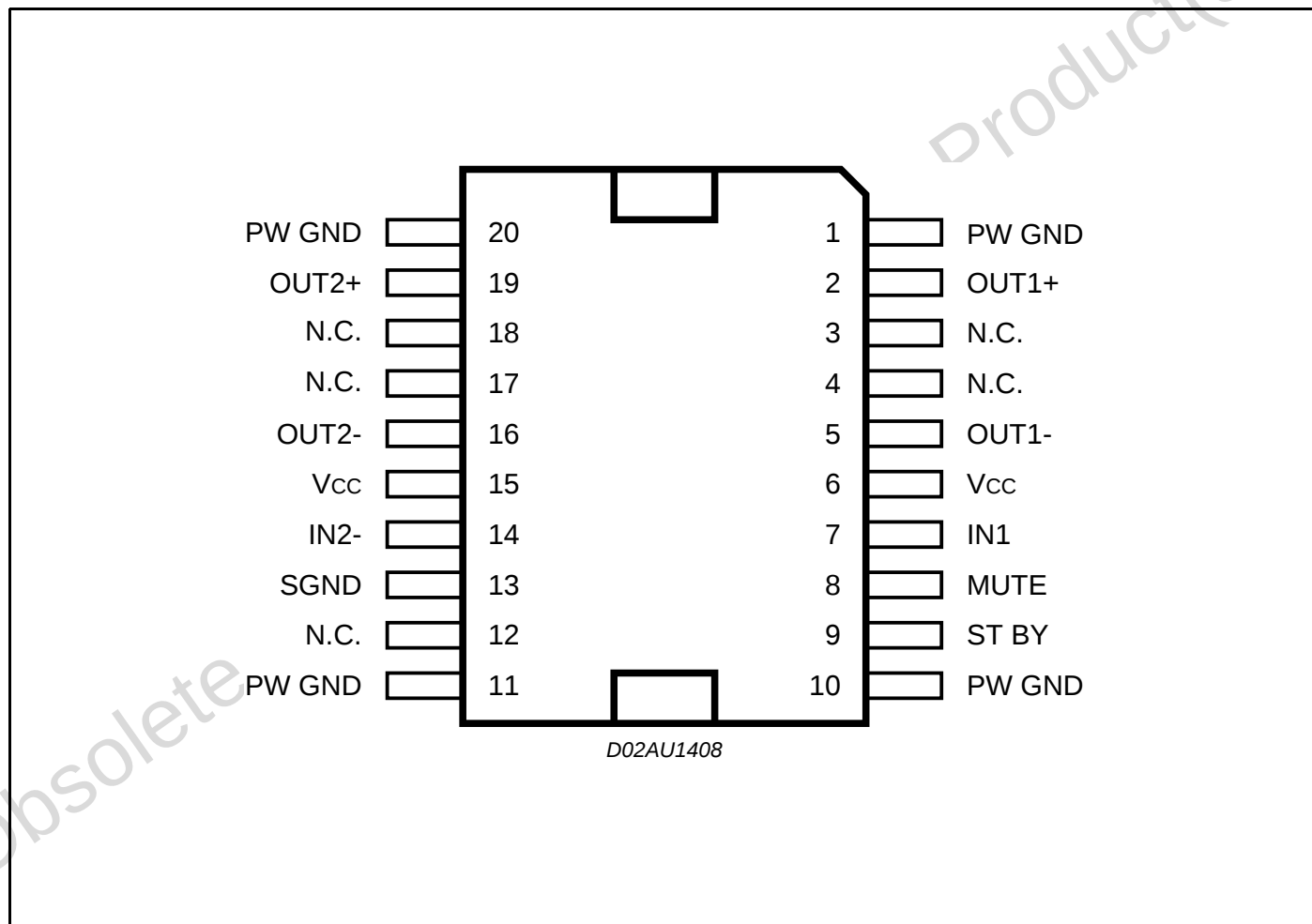
Figure 3. PIN CONNECTION
