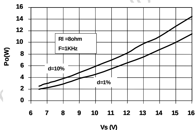
Figure 10. Output Power vs supply Voltage
