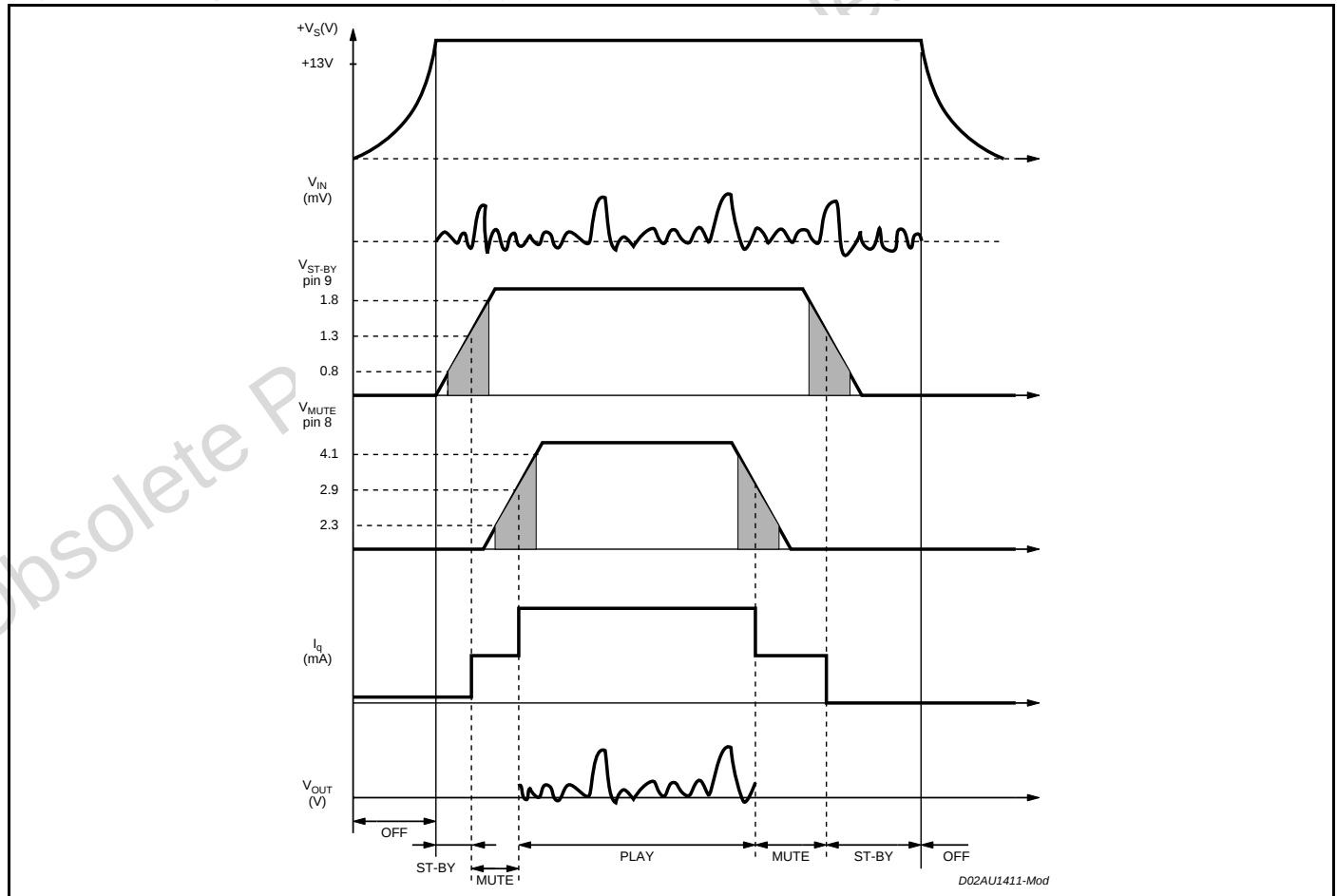
Figure 5. Microprocessor Driving Signals
