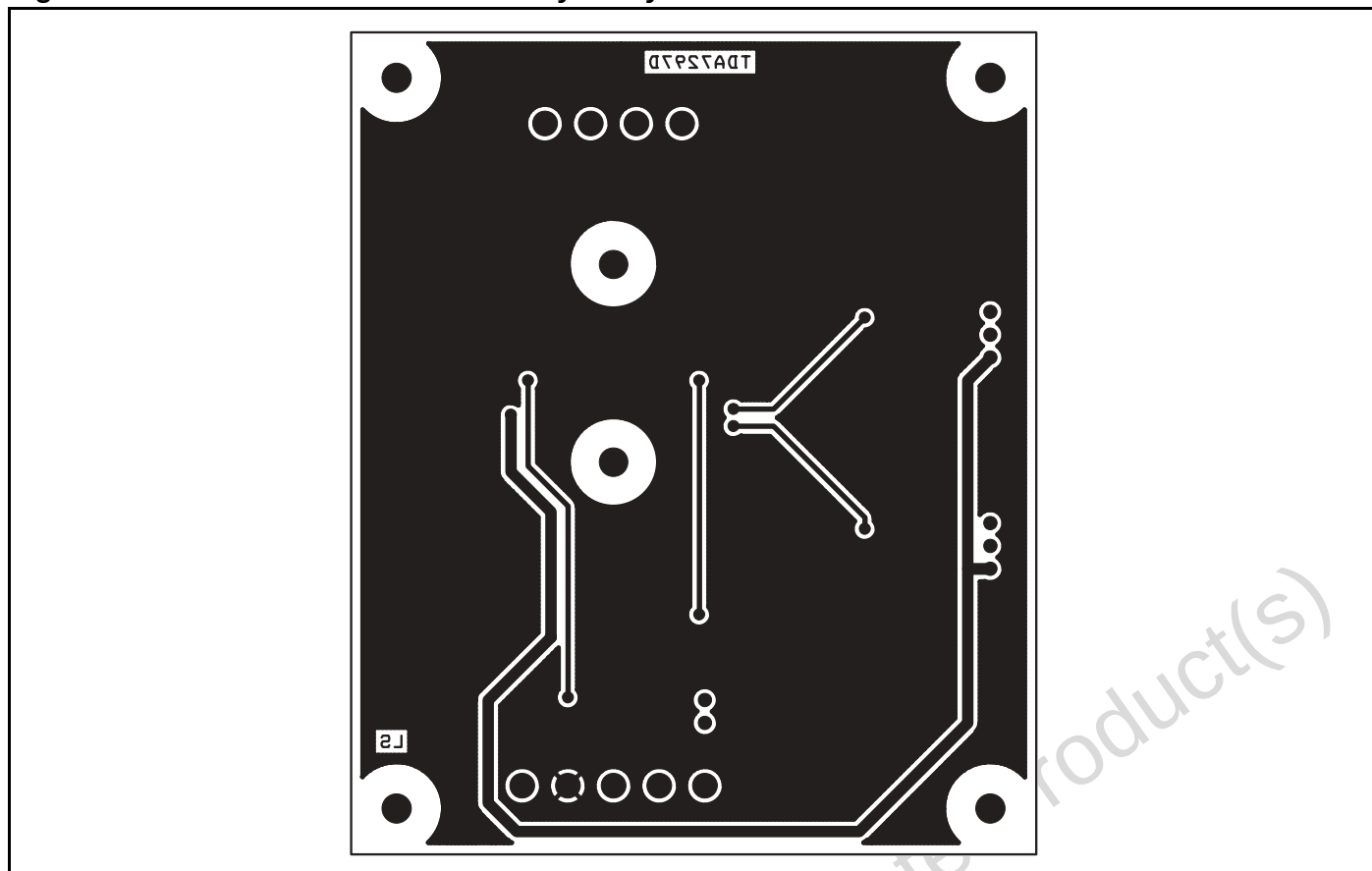
Figure 17. Evaluation Board Bottom Layer Layout
