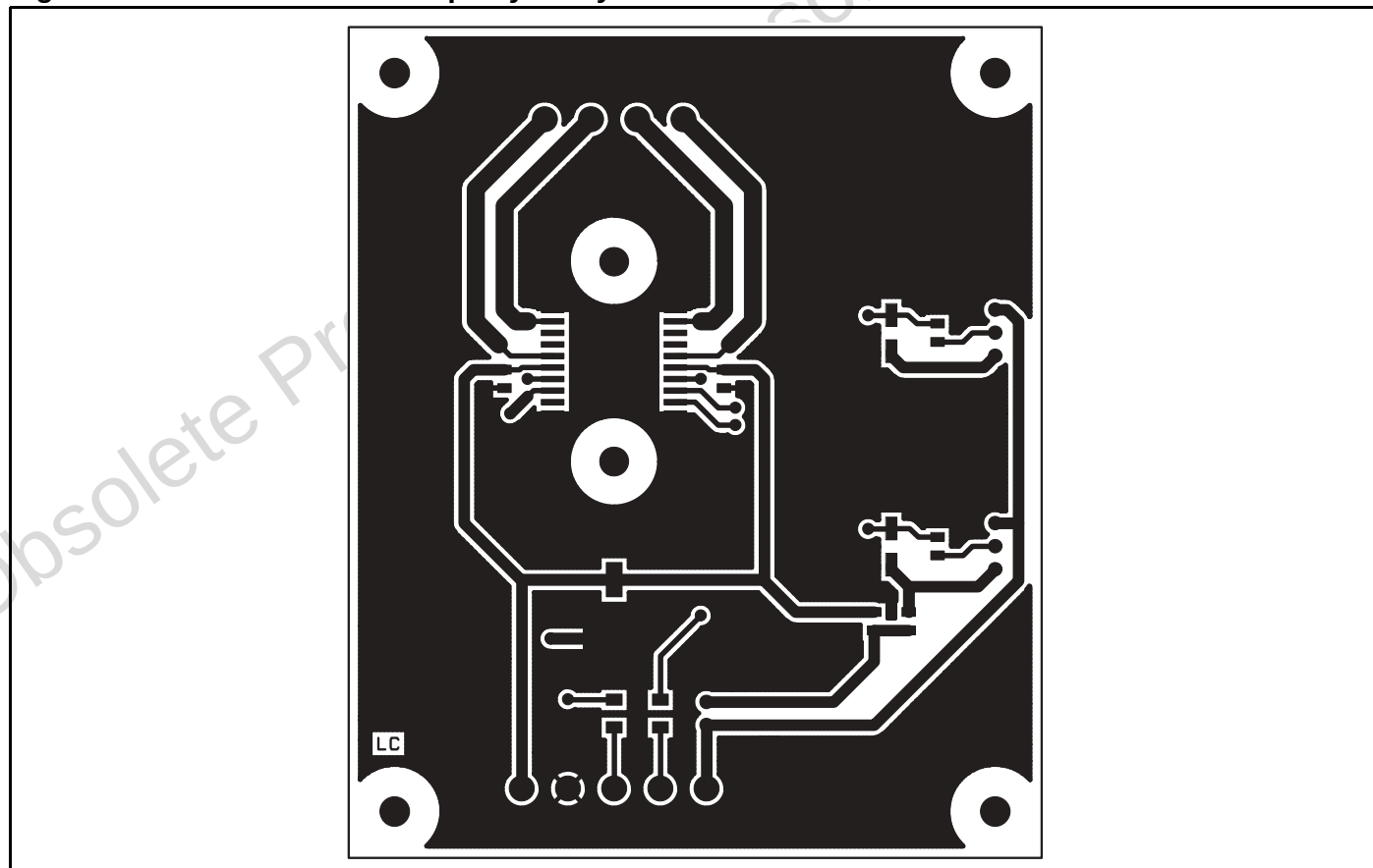
Figure 16. Evaluation Board Top Layer Layout
