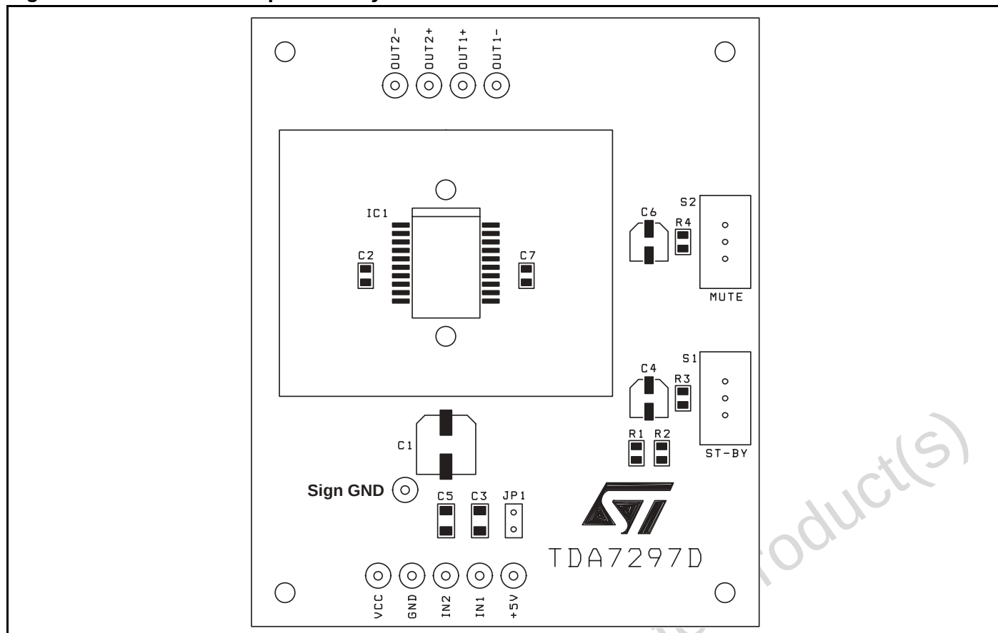
Figure 15. PC Board Component Layout
