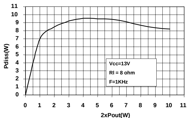
Figure 11. Power Dissipation vs Pout
