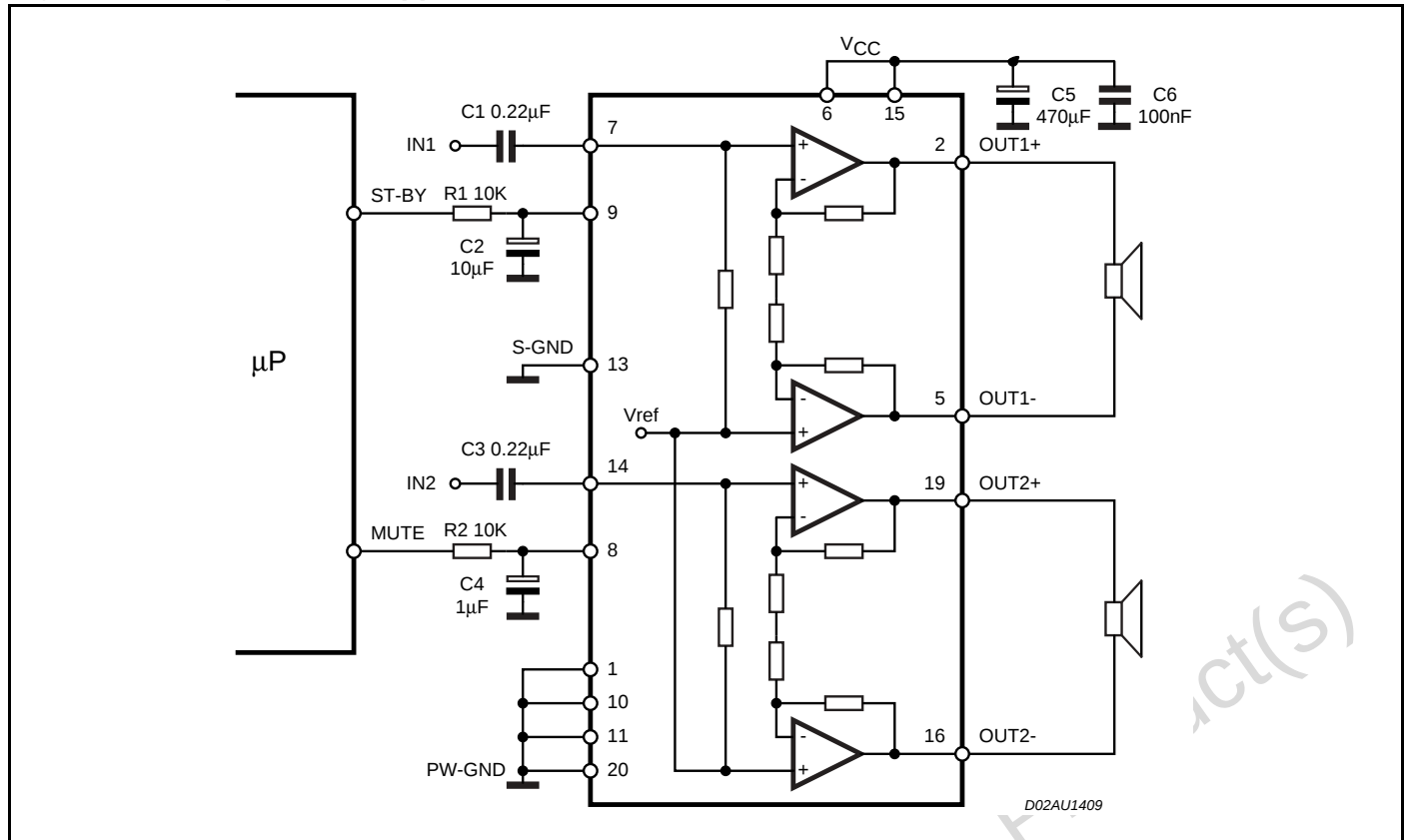
Figure 4. Microprocessor Application
