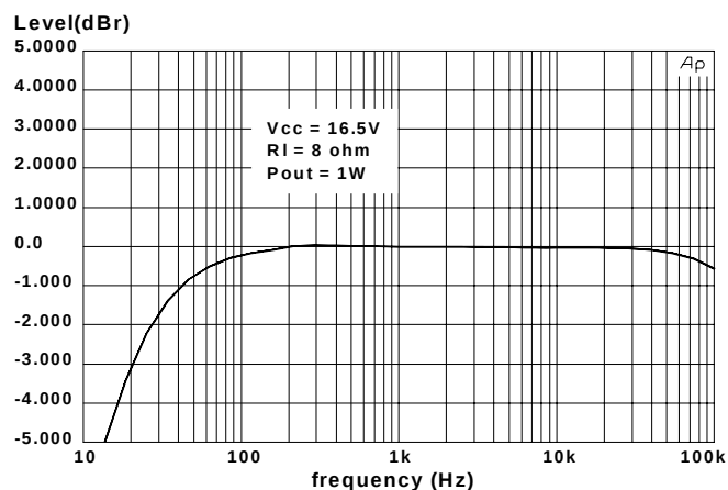
Figure 9. Frequency Response
