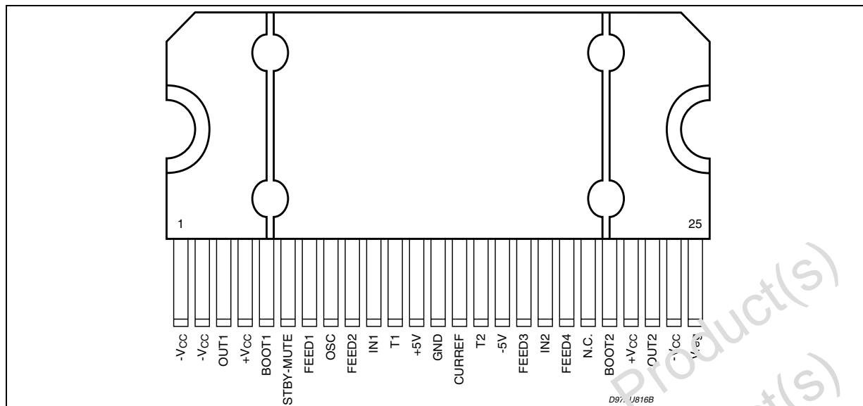
Figure 4. Pin Connection
