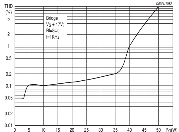
Figure 11. Distortion vs. Output Power in BTL
