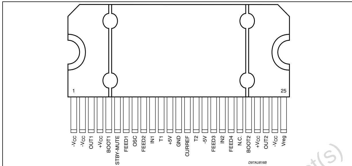
Figure 5. Pin Connection
