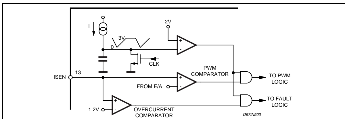
Figure 29. Internal LEB.
