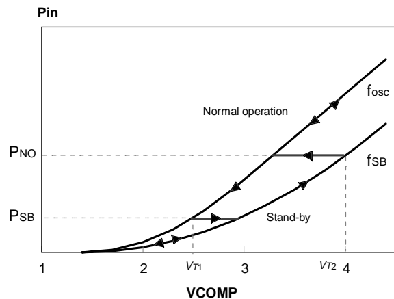
Figure 21. Standby dynamic operation.
