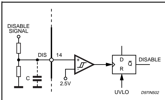
Figure 30. Disable (Latched).
