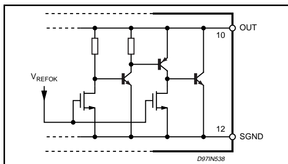
Figure 28. Pull-Down of the output in UVLO.
