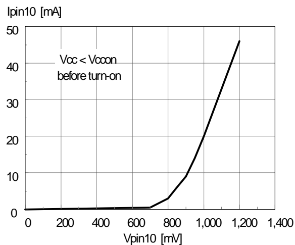
Figure 13. UVLO Saturation
