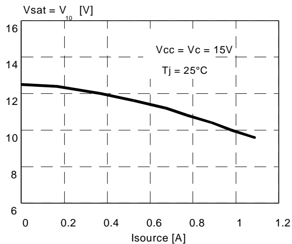
Figure 13. UVLO Saturation
