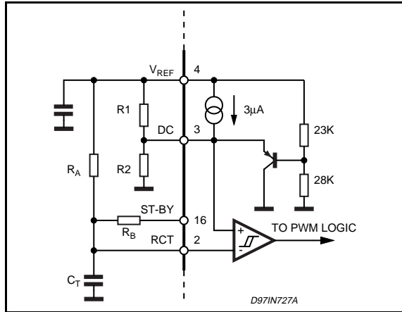
Figure 24. Duty cycle control.
