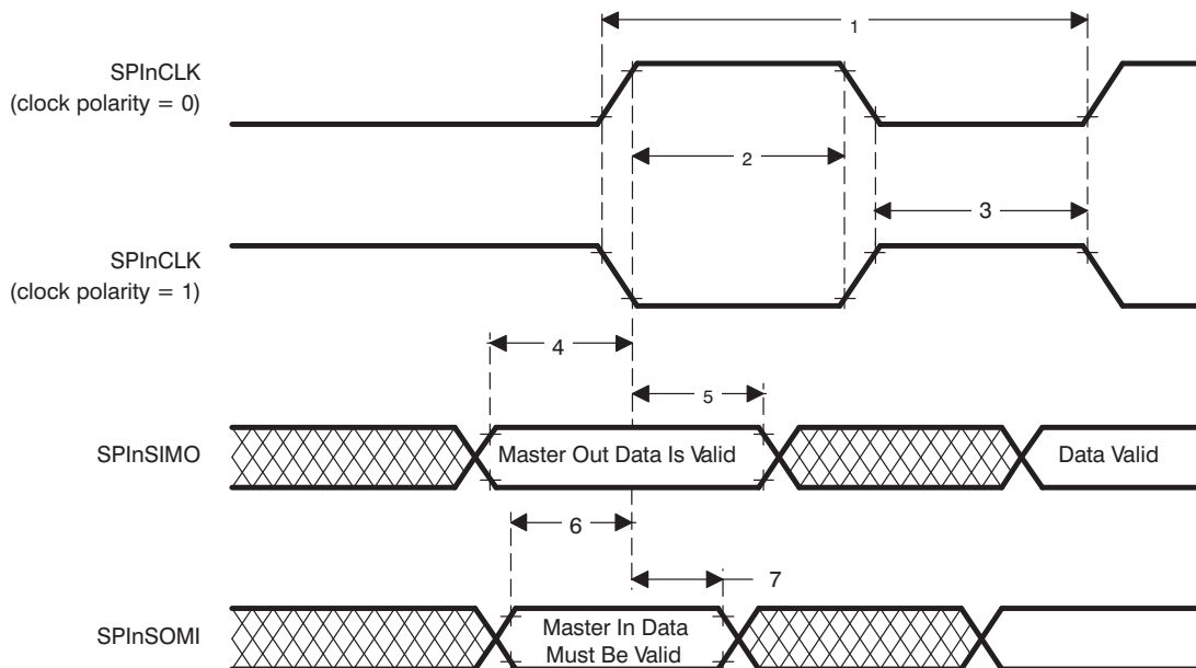
Figure 13. SPIn Master Mode External Timing (CLOCK PHASE = 1)
