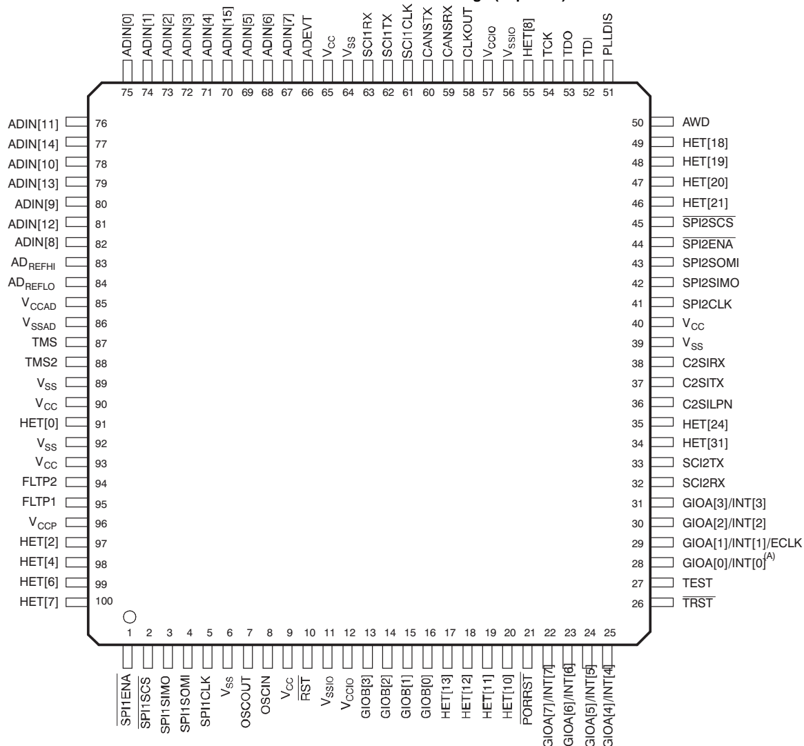
TMS470R1A128 100-Pin PZ Package (Top View)
