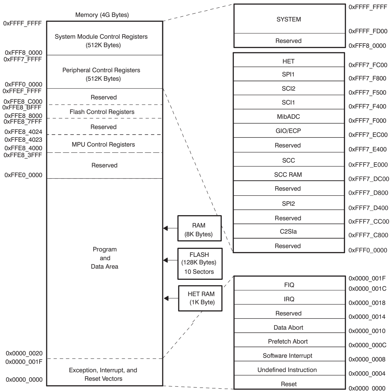
Figure 1. Memory Map
