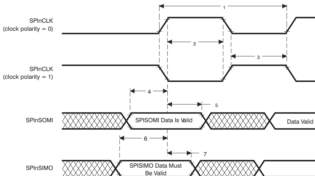
Figure 15. SPIn Slave Mode External Timing (CLOCK PHASE = 1)
