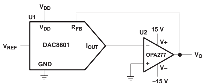
Figure 18. Voltage Output Configuration
