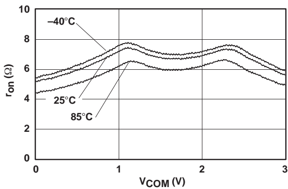
Figure 3. r_{on} vs V_{COM} ( V_+ = 3\text{ V} )
