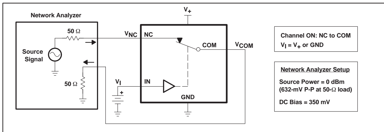
Figure 18. Bandwidth (BW)
