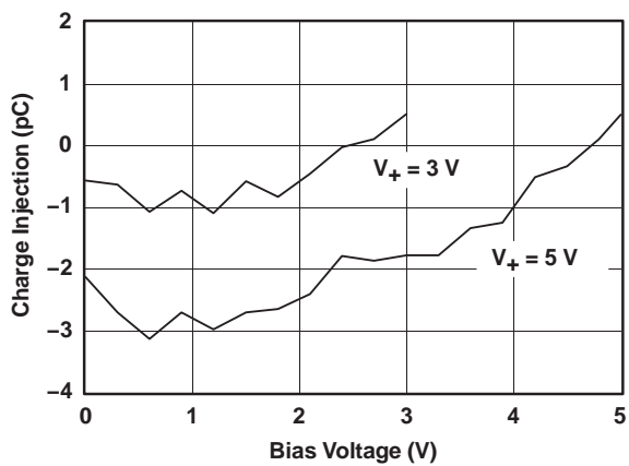
Figure 5. Charge-Injection ( Q_C ) vs V_{COM}
