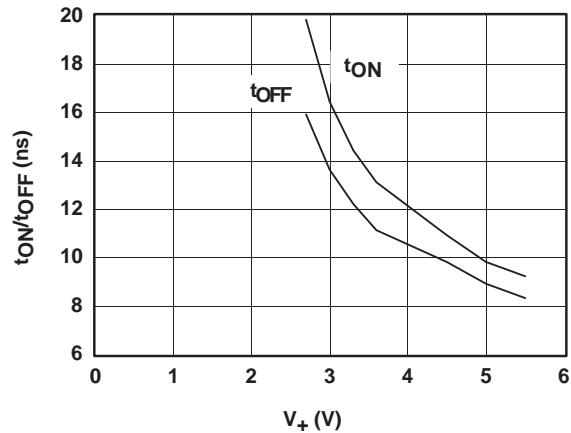
Figure 6. t_{ON} and t_{OFF} vs Supply Voltage
