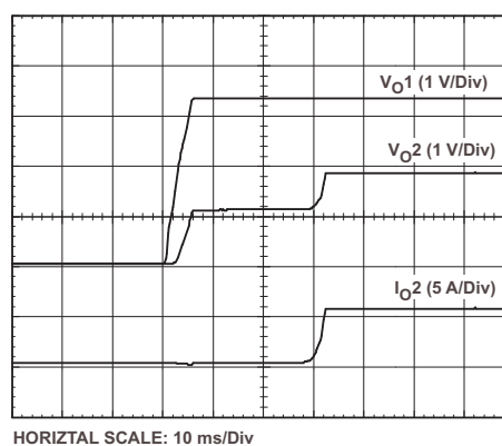
Figure 19. Pre-Bias Startup Waveforms
