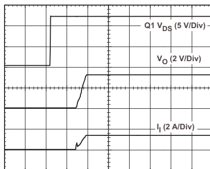
Figure 13. Power-Up from Inhibit Control
