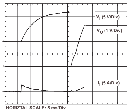
Figure 11. Power-Up Waveforms
