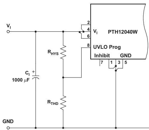
Figure 9. UVLO Program Resistor Placement
