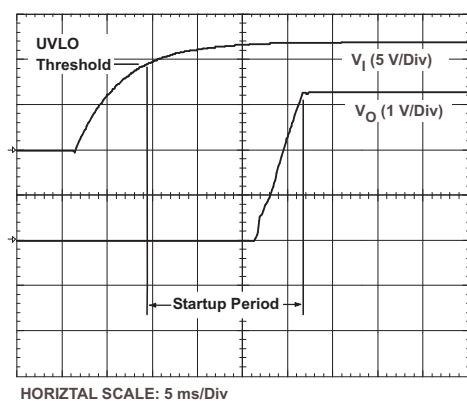
Figure 18. PTH12020W Startup
