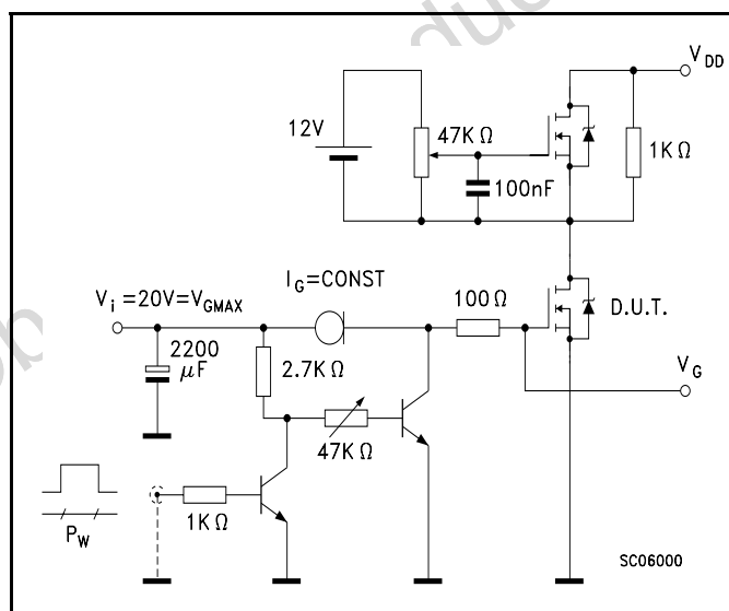
Figure 19: Gate Charge Test Circuit
