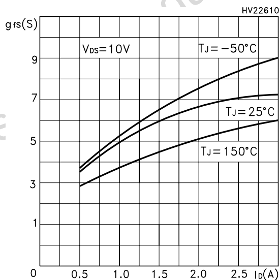
Figure 5: Transconductance
