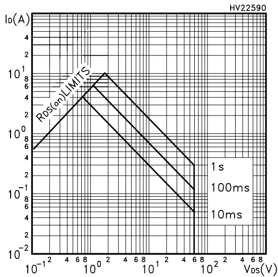
Figure 4: Output Characteristics
