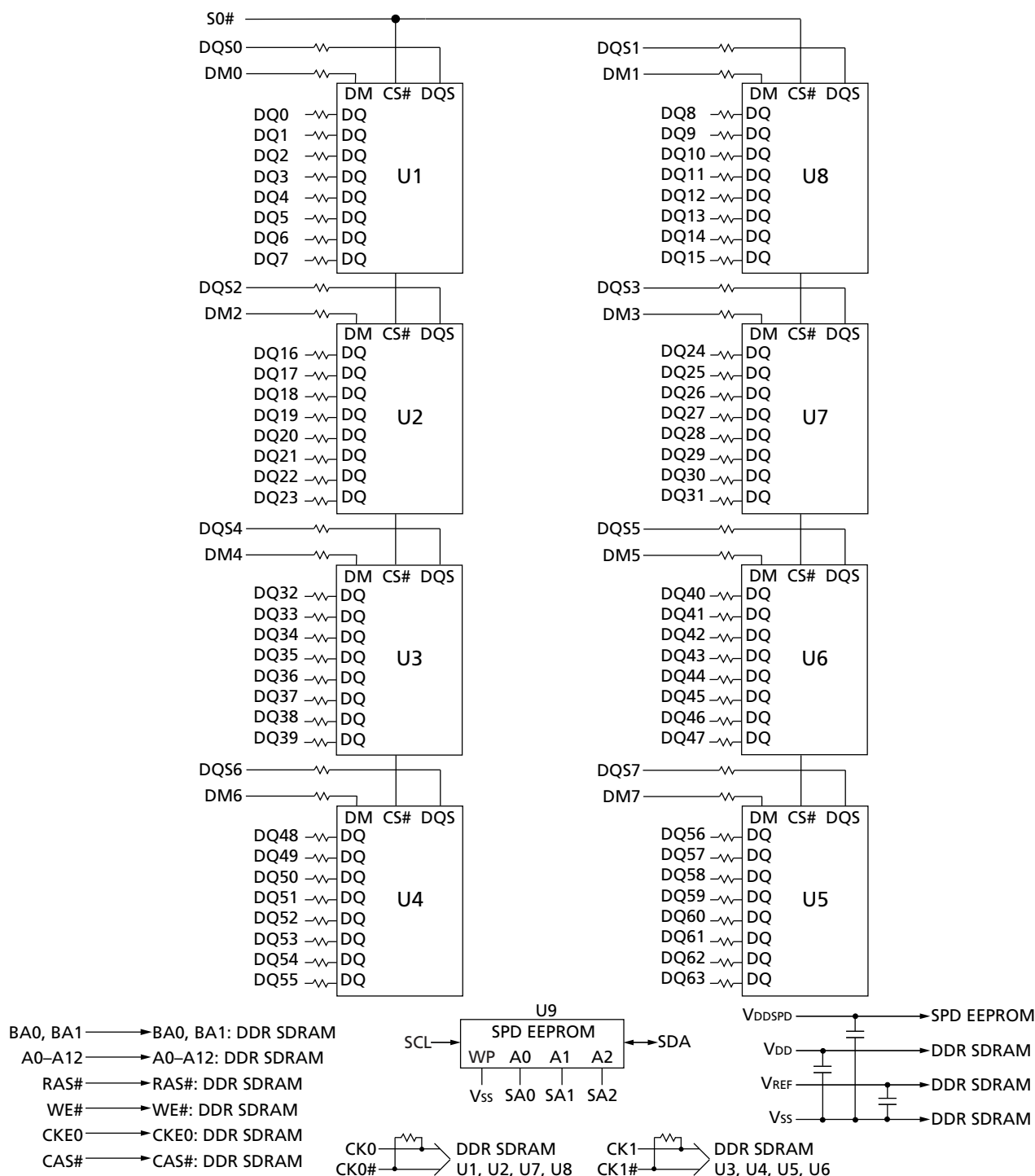
Figure 3: Functional Block Diagram – Layout 2 (256MB, 512MB)
