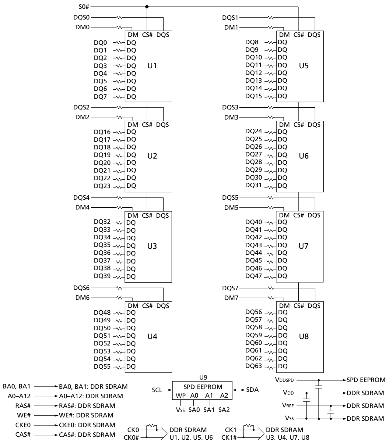
Figure 2: Functional Block Diagram – Layout 1 (256MB)
