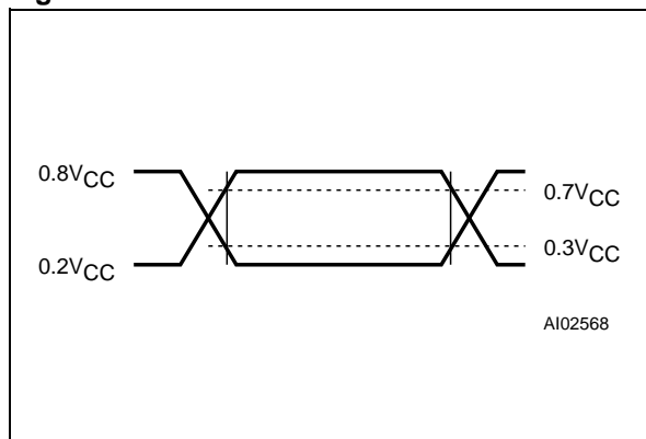
Figure 12. AC Measurement I/O Waveform
