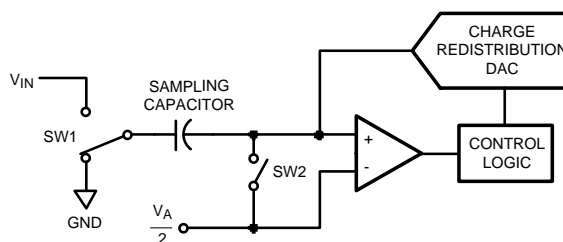
Figure 19. ADC081S101 in Hold Mode
