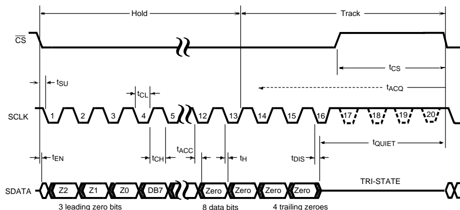
Figure 3. ADC081S101 Serial Timing Diagram
