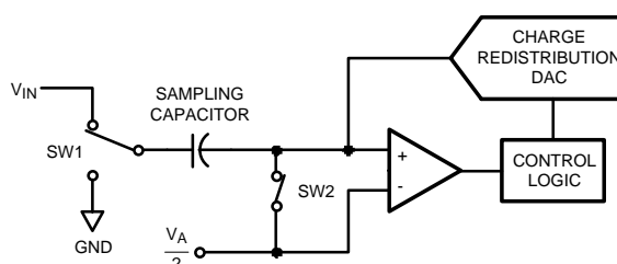
Figure 18. ADC081S101 in Track Mode
