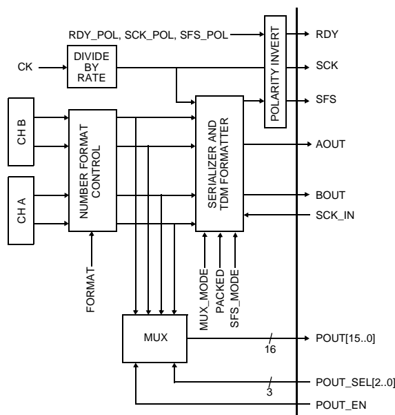
Figure 29. CLC5903 output circuit
