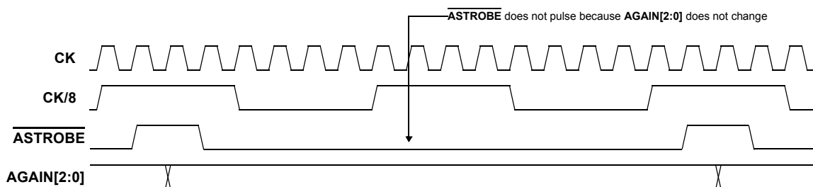
Figure 35. Timing diagram for AGC/DVGA interface, Channel A. Refer to Figure 9 for detailed timing information.
