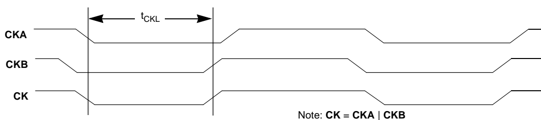
Figure 8. CLC5903 CKA vs. CKB Timing
