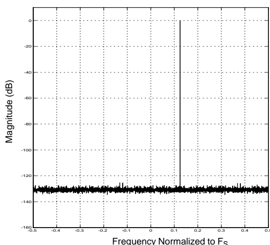
(b) After Phase Dithering
