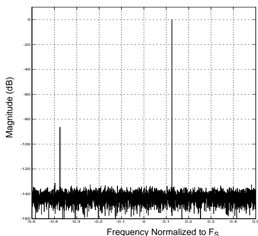
(a) Before Phase Dithering
