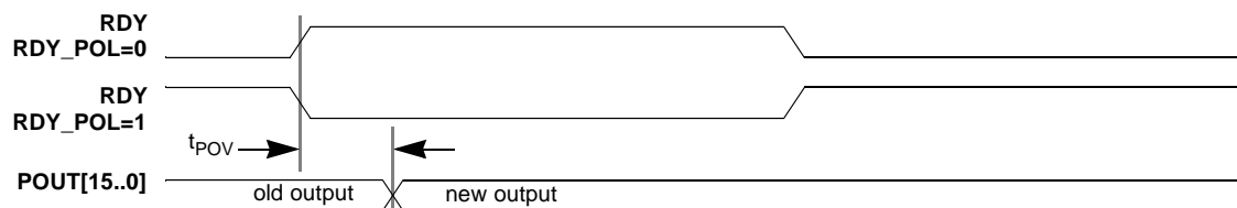
Figure 13. CLC5903 Parallel Output Data Ready Timing
