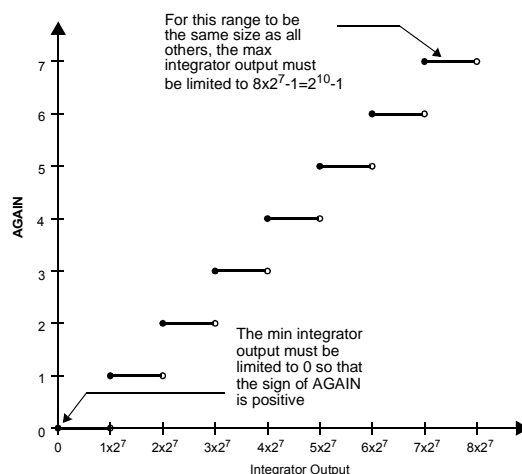
Figure 38. AGC integrator output limits
