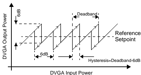
Figure 33. AGC Setup.
