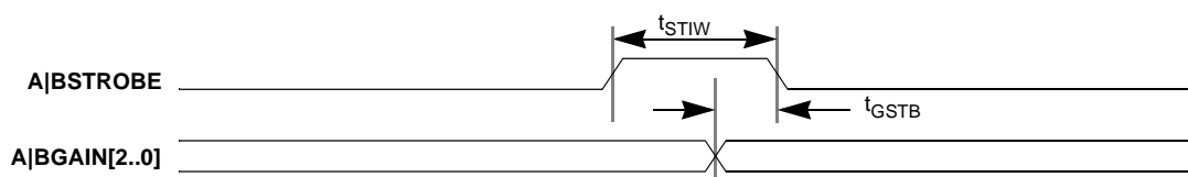
Figure 9. CLC5903 DVGA Interface Timing
