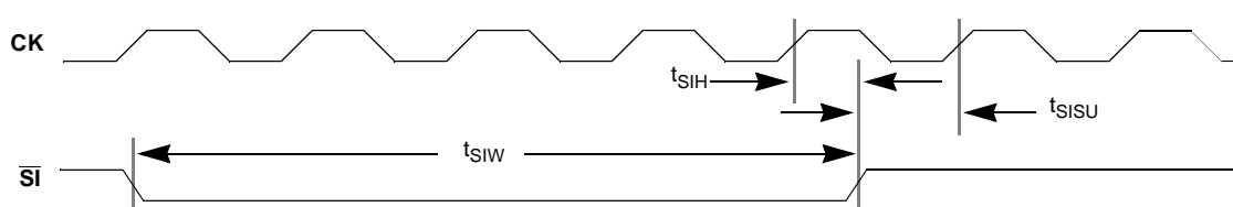
Figure 6. CLC5903 Synchronization Input (SI) Timing
