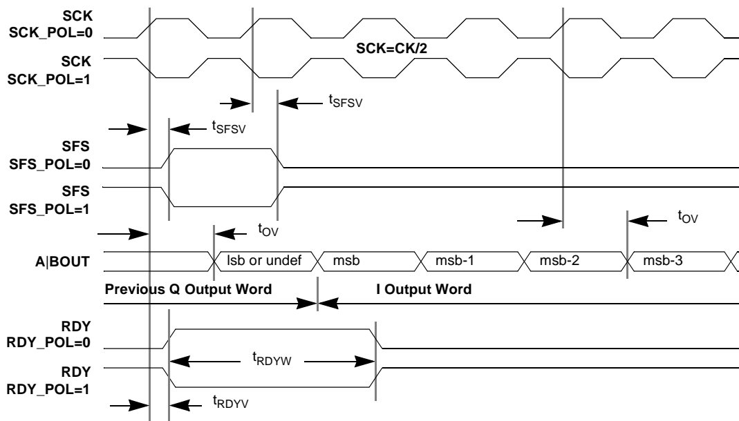
Figure 10. CLC5903 Serial Port Timing
