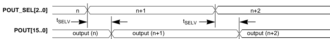
Figure 12. CLC5903 Parallel Output Select Timing
