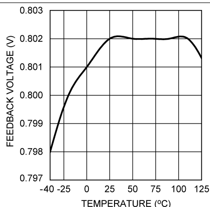
Figure 5. V_{FB} vs Temperature
