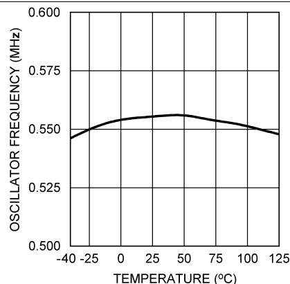
Figure 2. Oscillator Frequency vs Temperature - L1 = 10\text{ }\mu\text{H}
