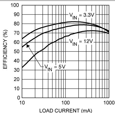
Figure 22. Efficiency vs Load Current - L1 = 10 µH V OUT = 1.5 V
