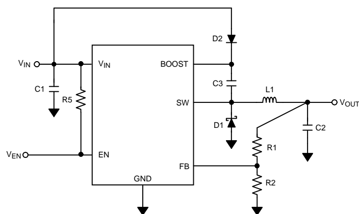
Figure 33. Layout Schematic
