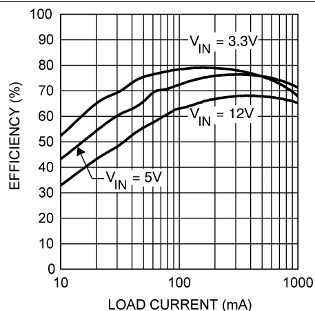
Figure 21. Efficiency vs Load Current - L1 = 4.7 µH V OUT = 1.5 V
