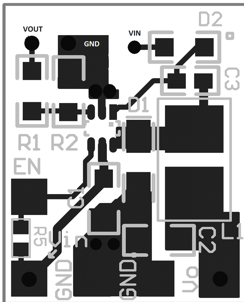
Figure 32. Top Layer
