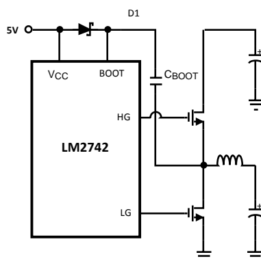
Figure 29. BOOT Supplied by Charge Pump
