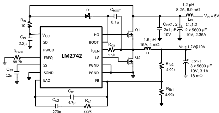
Figure 32. 5V to 1.2V, 10A, 300kHz
