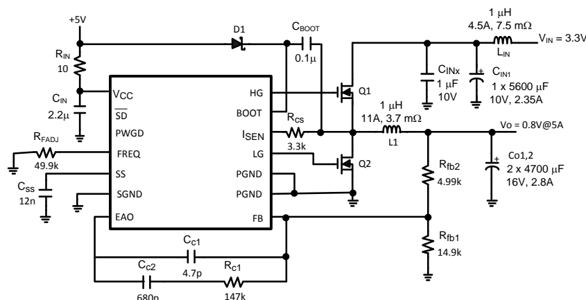
Figure 34. 3.3V to 0.8V, 5A, 500kHz
