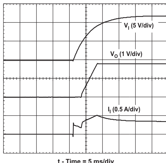
Figure 11. Power-Up Waveforms
