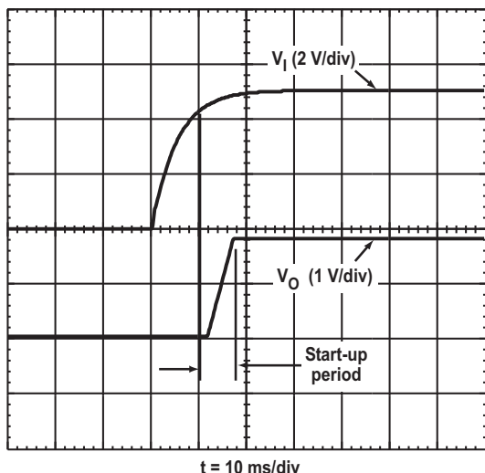
Figure 14. PTV05020W Start-Up
