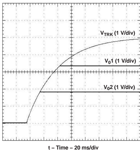
Figure 12. Simultaneous Power Up With Auto-Track Control
