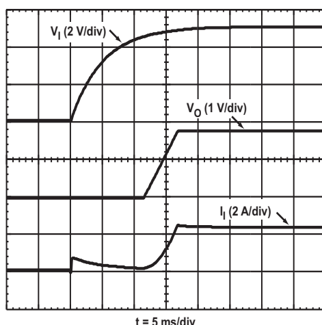
Figure 8. Power-Up Waveforms
