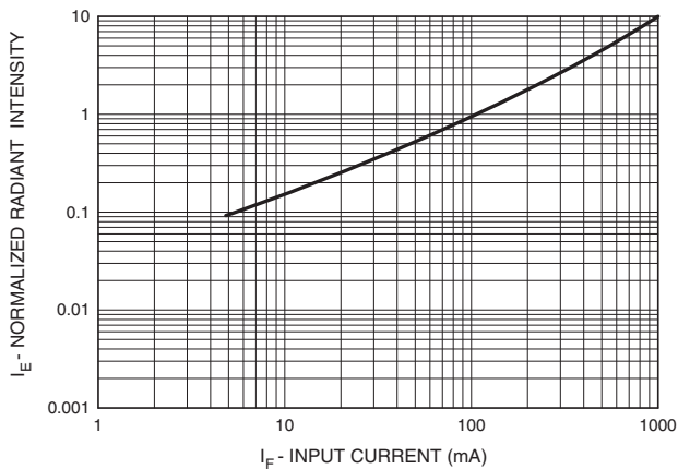
Fig.1 Relative Radiant Intensity vs. Input Current
