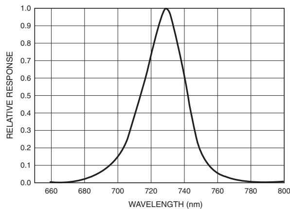
Fig.5 Spectral Response
