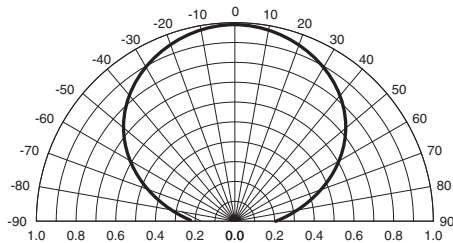
Fig.3 Radiation Diagram
