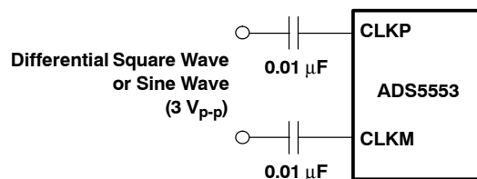
Figure 35. AC-Coupled, Differential Clock Input
