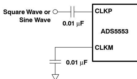
Figure 34. AC-Coupled, Single-Ended Clock Input
