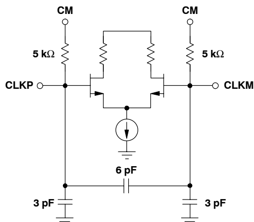
Figure 33. Clock Inputs
