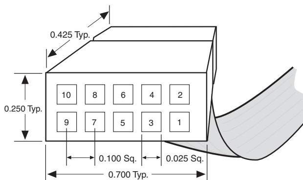
Figure 2-2. ByteBlaster II 10-Pin Female Plug Dimensions
