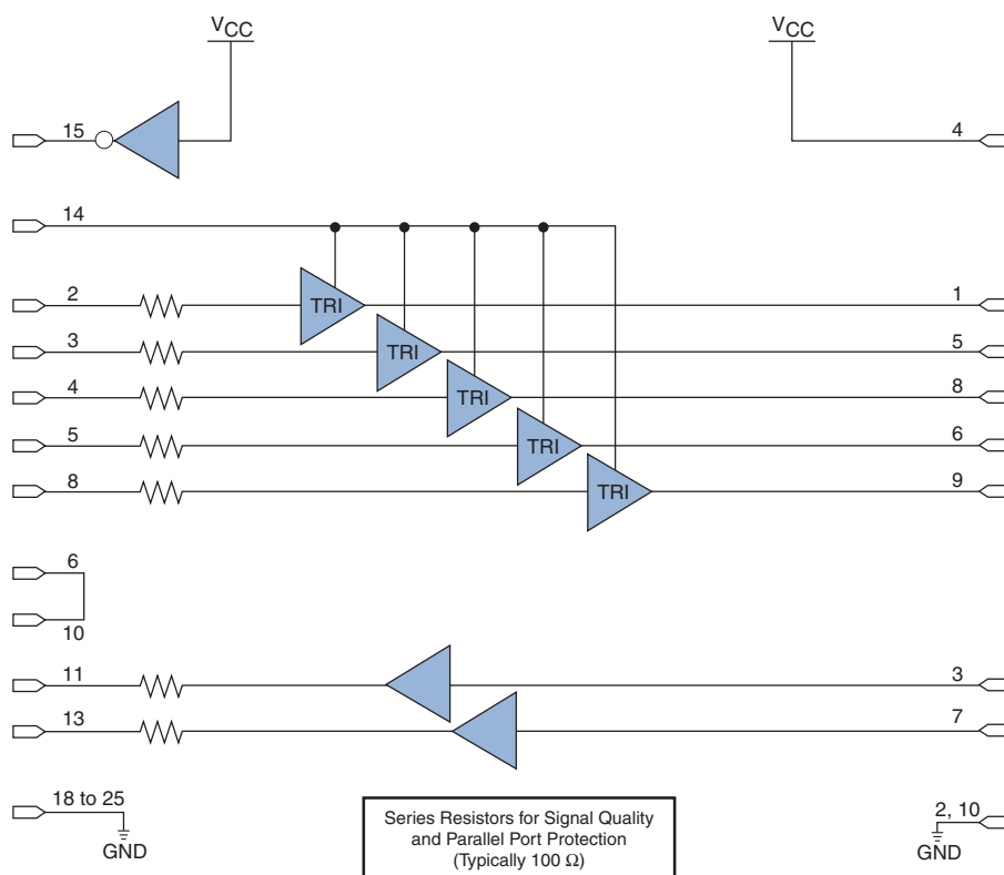
Figure 2-1. ByteBlaster II Block Diagram
