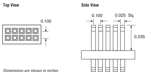
Figure 2-3. 10-Pin Male Header Dimensions
