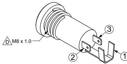
HOUSING DETAIL DRAWING
