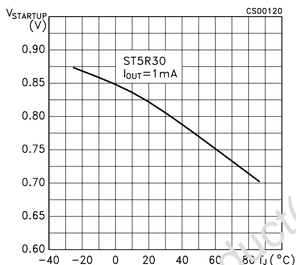
Figure 21: Start-up Voltage (V IN - V F ) vs Temperature
