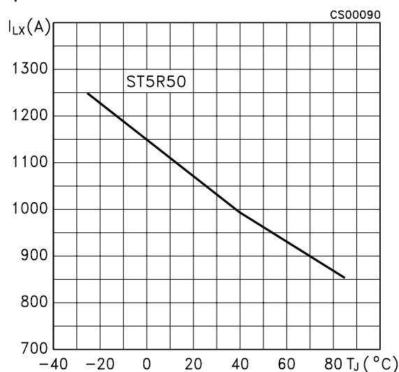
Figure 18: LX Switching Current Limit vs Temperature
