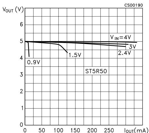
Figure 7: Output Voltage vs Output Current
