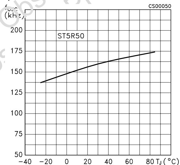
Figure 14: Maximum Oscillator Frequency vs Temperature
