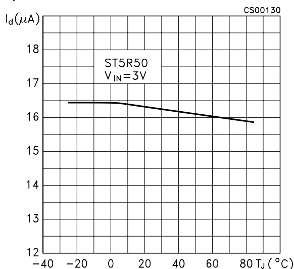
Figure 30: No Load Input Current vs Temperature
