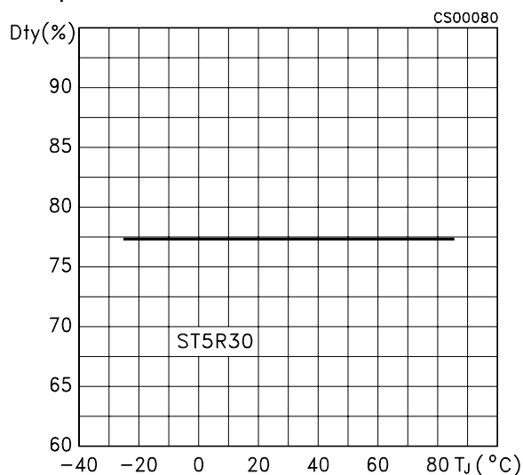
Figure 17: Oscillator Duty Cycle (@ MAX Freq.) vs Temperature
