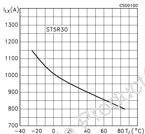
Figure 19: LX Switching Current Limit vs Temperature
