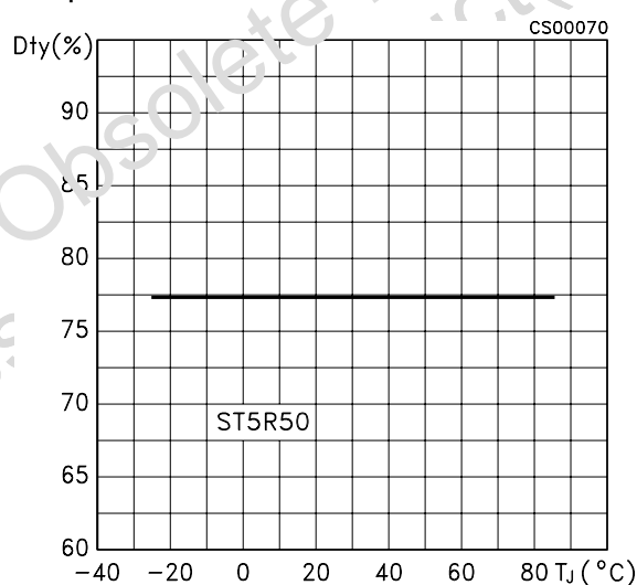
Figure 16: Oscillator Duty Cycle (@ MAX Freq.) vs Temperature
