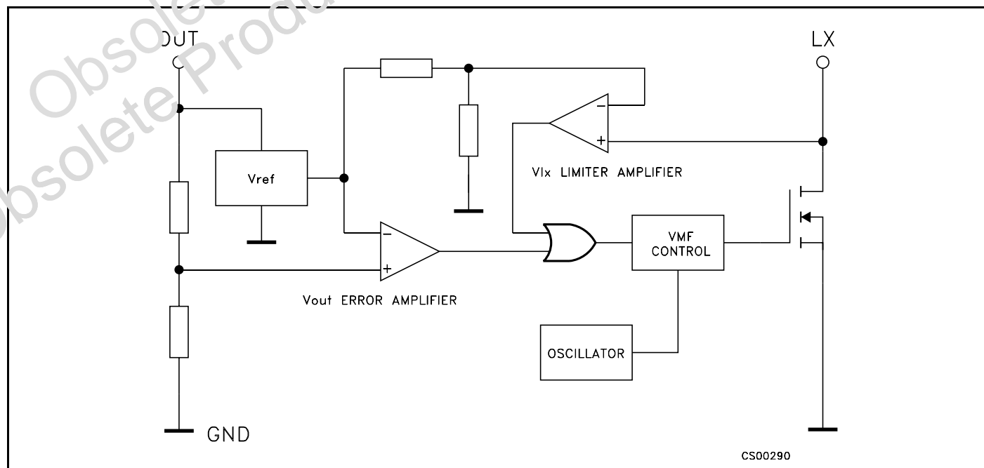
Figure 1: Schematic Diagram
