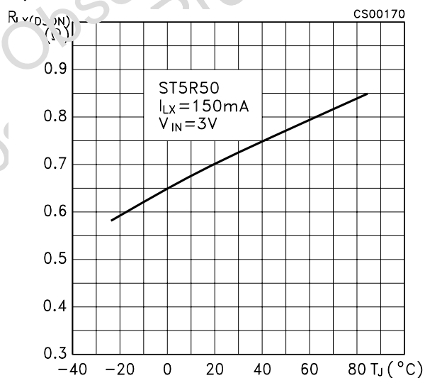
Figure 26: Internal Switch R_{DS(on)} vs Temperature
