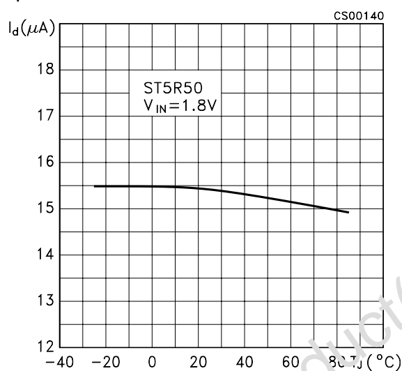
Figure 31: No Load Input Current vs Temperature
