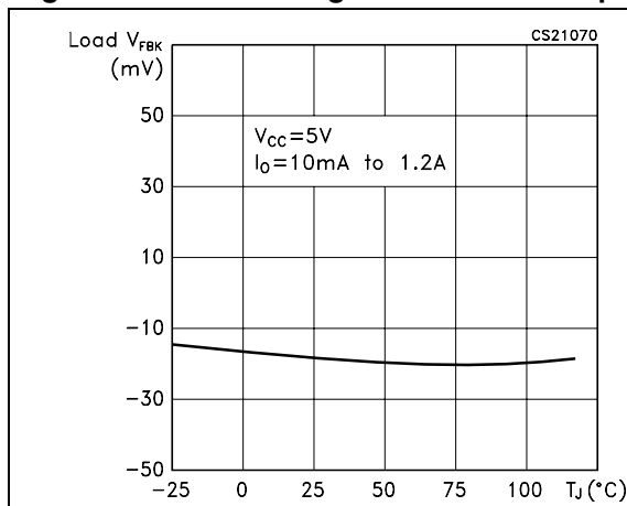
Figure 4. Load voltage feedback vs temp.
