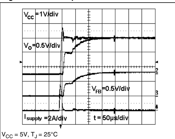
Figure 21. Start-Up transient
