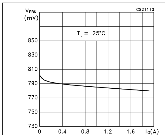
Figure 8. Voltage feedback vs output current
