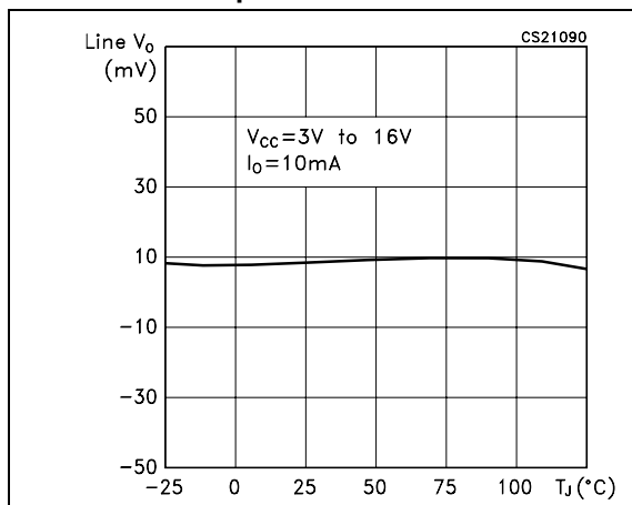
Figure 6. Line output voltage regulation vs temperature
