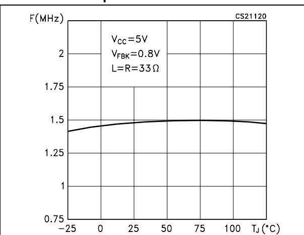
Figure 9. PWM Switching frequency vs temperature
