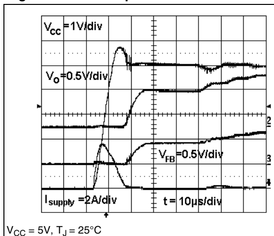
Figure 20. Start-Up transient
