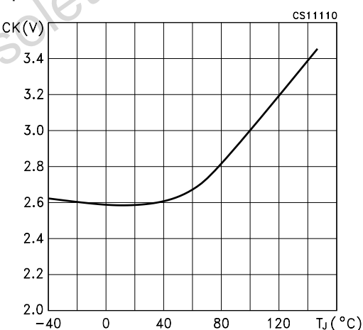
Figure 6 : INHIBIT Threshold Voltage vs Temperature
