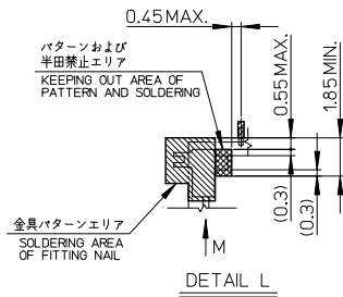
DETAIL L
