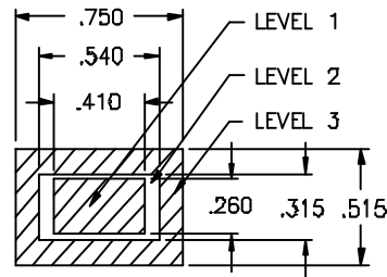
REQUIRED FOOTPRINT
