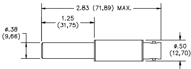
STANDARD WECC/BNC ADAPTER (4X MODEL 5008)
