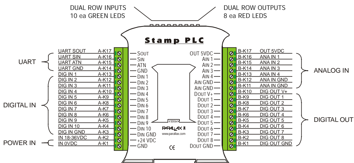
Figure 11: Connection Diagram
