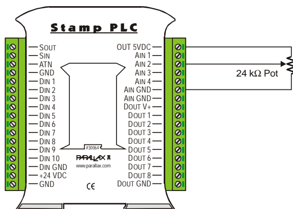
Figure 9: Stamp PLC to Potentiometer
