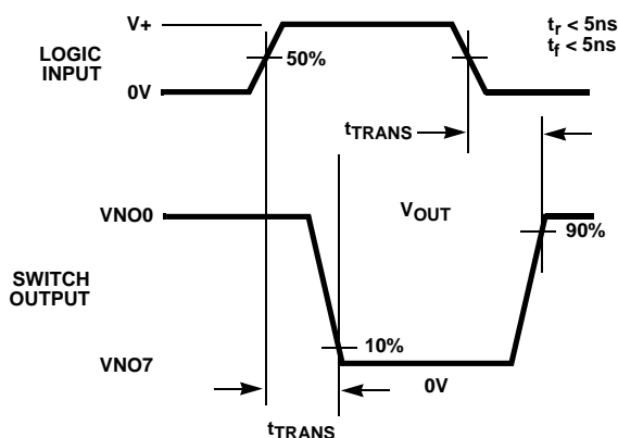
FIGURE 1C. ADDRESS t_{TRANS} MEASUREMENT POINTS
