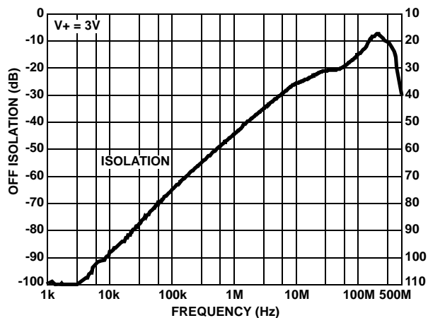
FIGURE 17. OFF-ISOLATION
