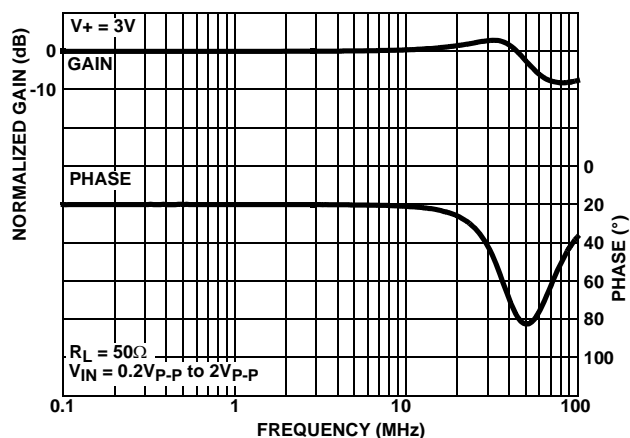
FIGURE 16. FREQUENCY RESPONSE
