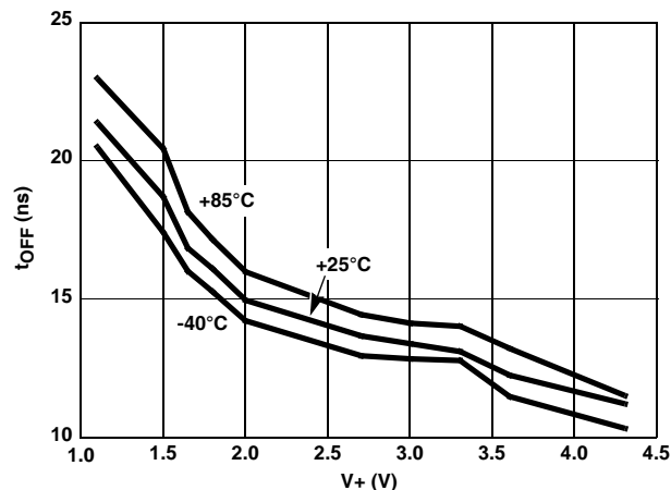
FIGURE 15. INHIBIT TURN-OFF TIME vs SUPPLY VOLTAGE
