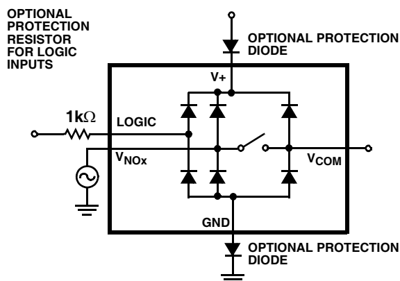
FIGURE 7. OVERVOLTAGE PROTECTION
