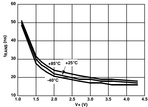
FIGURE 13. ADDRESS TRANS TIME vs SUPPLY VOLTAGE
