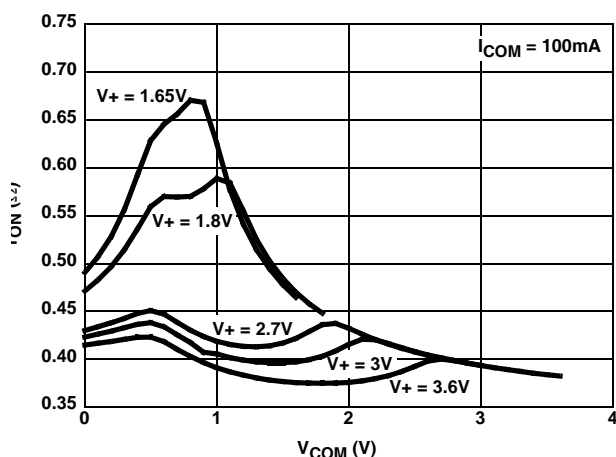
FIGURE 8. ON-RESISTANCE vs SUPPLY VOLTAGE vs SWITCH VOLTAGE
