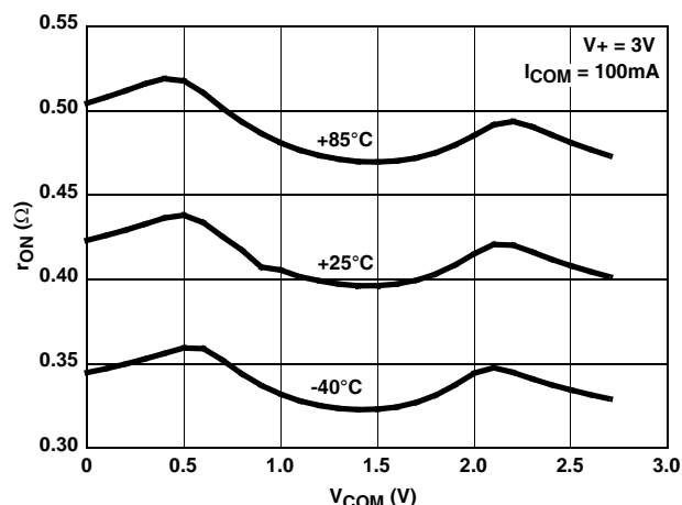
FIGURE 9. ON-RESISTANCE vs SWITCH VOLTAGE
