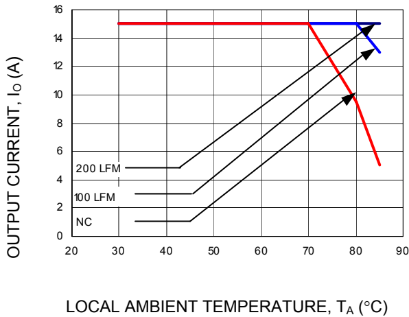
Figure 3. Derating curves for QW015A0F1-H (Vo = 3.3V) in transverse orientation (Vin = 48Vdc)
