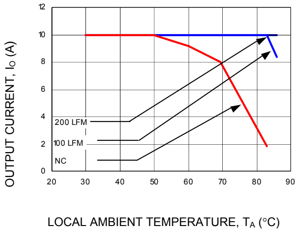
Figure 2. Derating curves for QW010A0A1-H (Vo = 5.0) in transverse orientation (Vin = 48Vdc)
