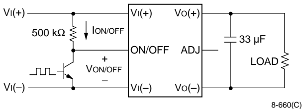
Figure 3. External Remote On/Off Circuitry
