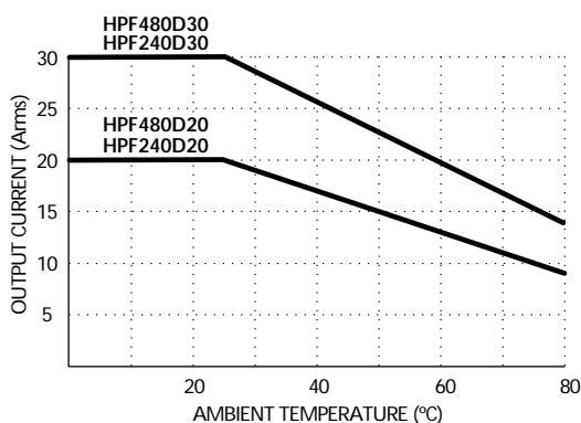
HPF Max. Output Current vs. Temp.
