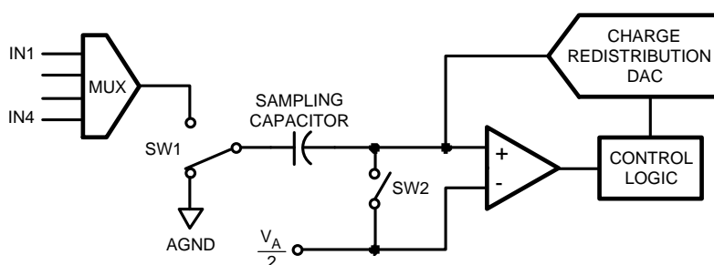
Figure 47. ADC124S021 in Hold Mode
