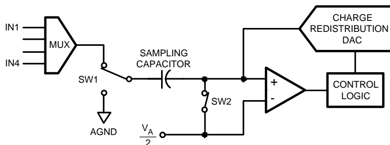
Figure 46. ADC124S021 in Track Mode
