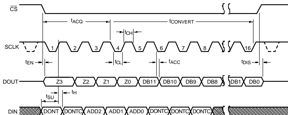
Figure 4. ADC124S021 Serial Timing Diagram
