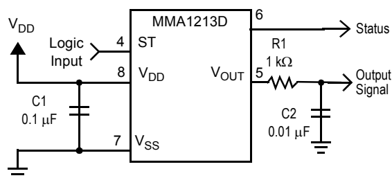
Figure 4. Accelerometer with Recommended Connection Diagram
