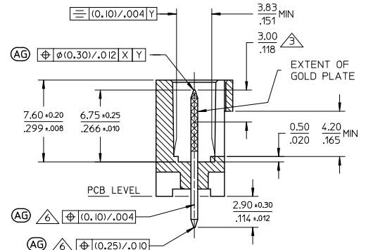
SECTION Z-Z
