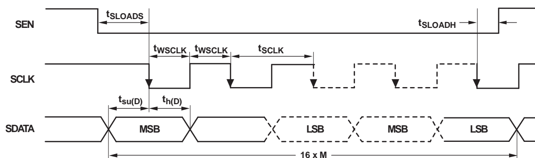
Figure 4. Serial Programming Interface Timing Diagram
