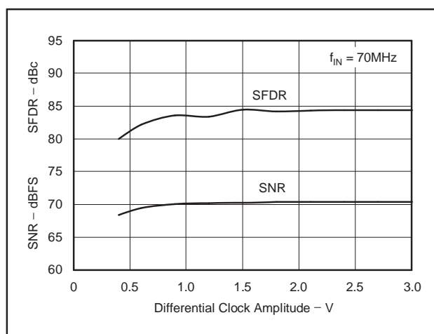
Figure 49. AC Performance vs Clock Amplitude
