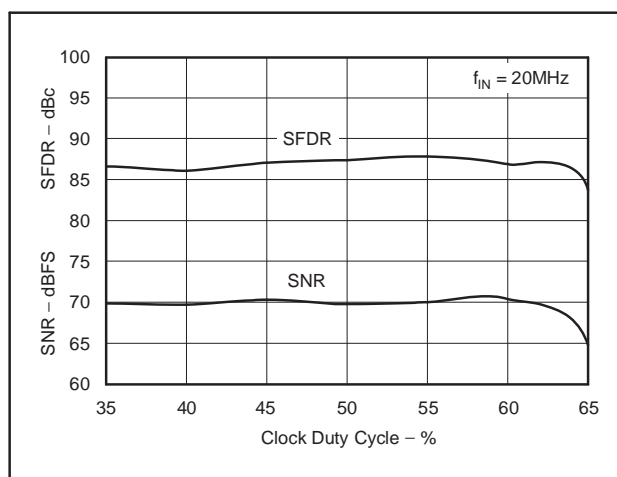
Figure 48. AC Performance vs Clock Duty Cycle
