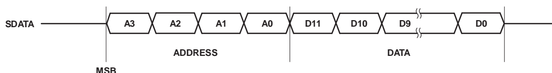
Figure 3. DATA Communication is 2-Byte, MSB First
