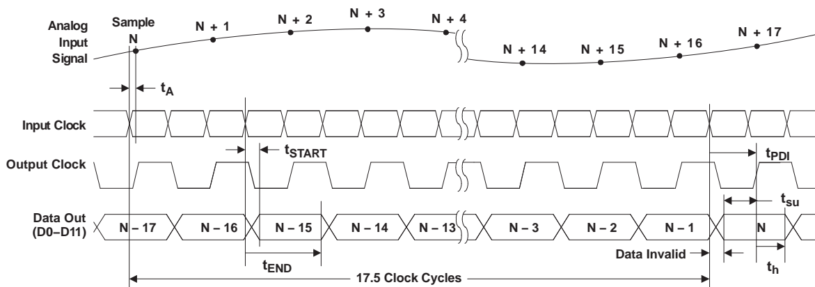
Figure 1. Timing Diagram
