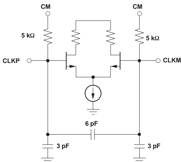
Figure 45. Clock Inputs
